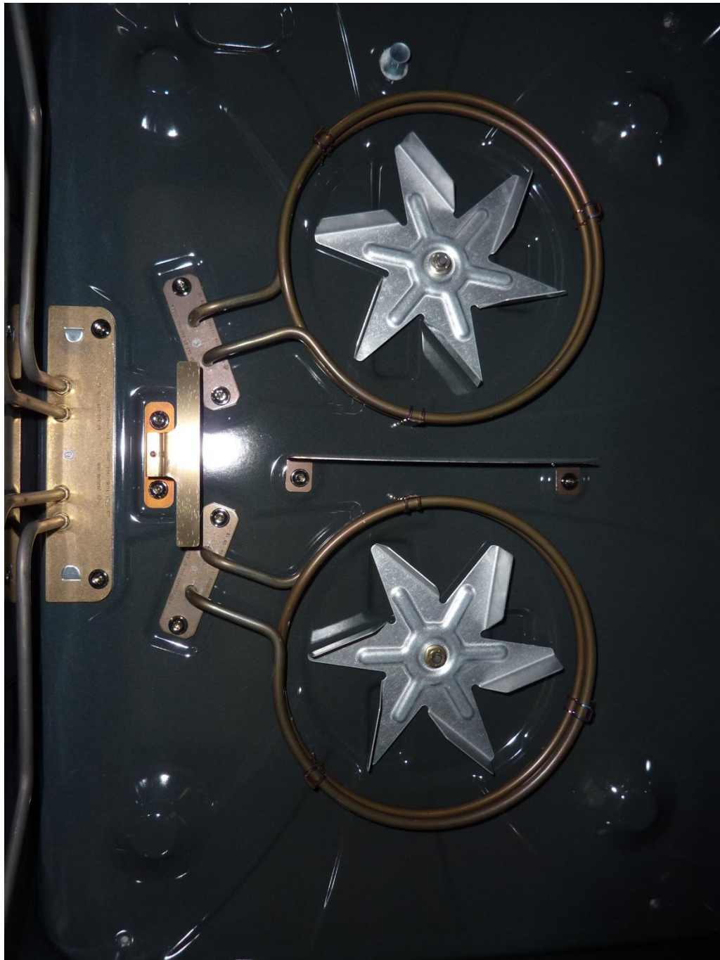
132604_2_k.JPG: EPI7674 inside H6880BP, antenna view
