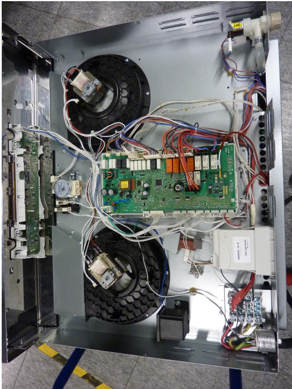
132604_2_d.JPG: EPI7674 inside H6880BP, internal view 1 (cover removed)
