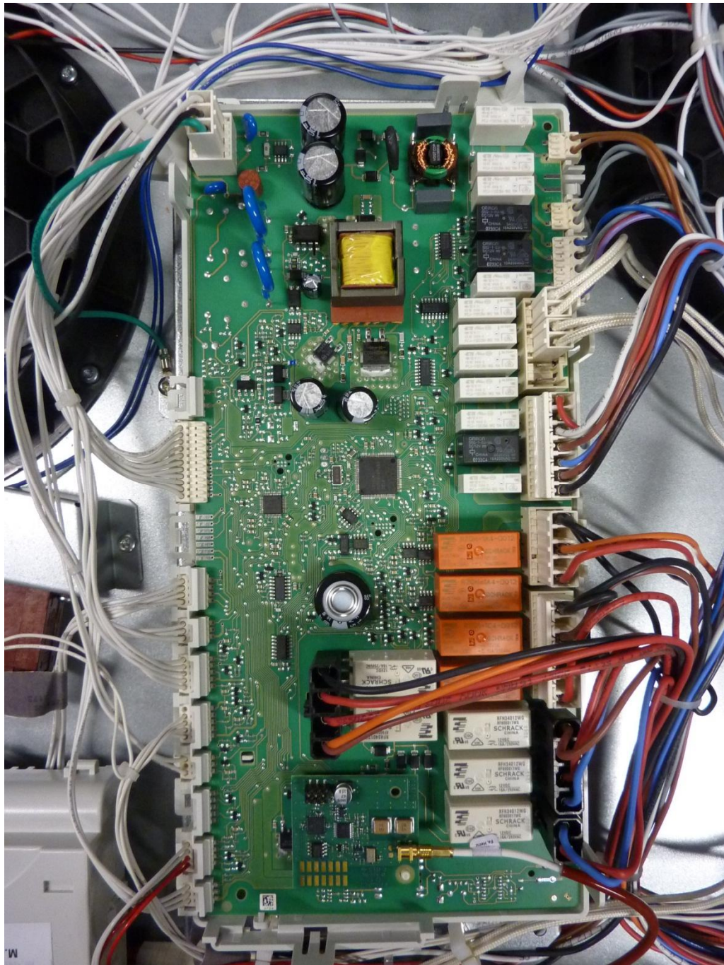
132604_2_e.JPG: EPI7674 inside H6880BP, internal view to main PCB
