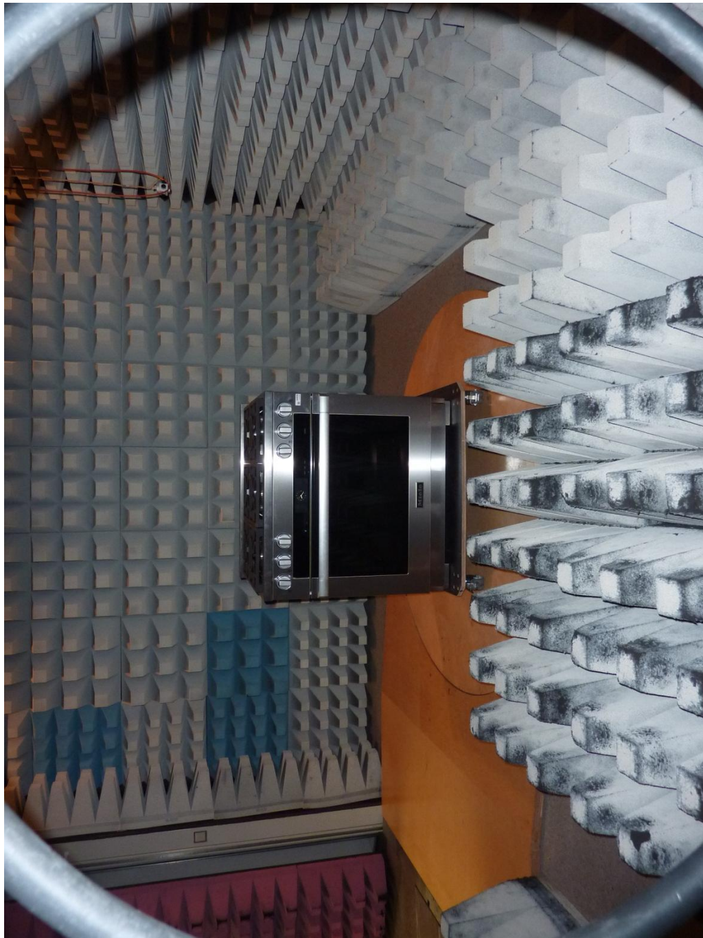
136015_2_6.JPG: EPI7674 inside HR1934, test set-up fully anechoic chamber
