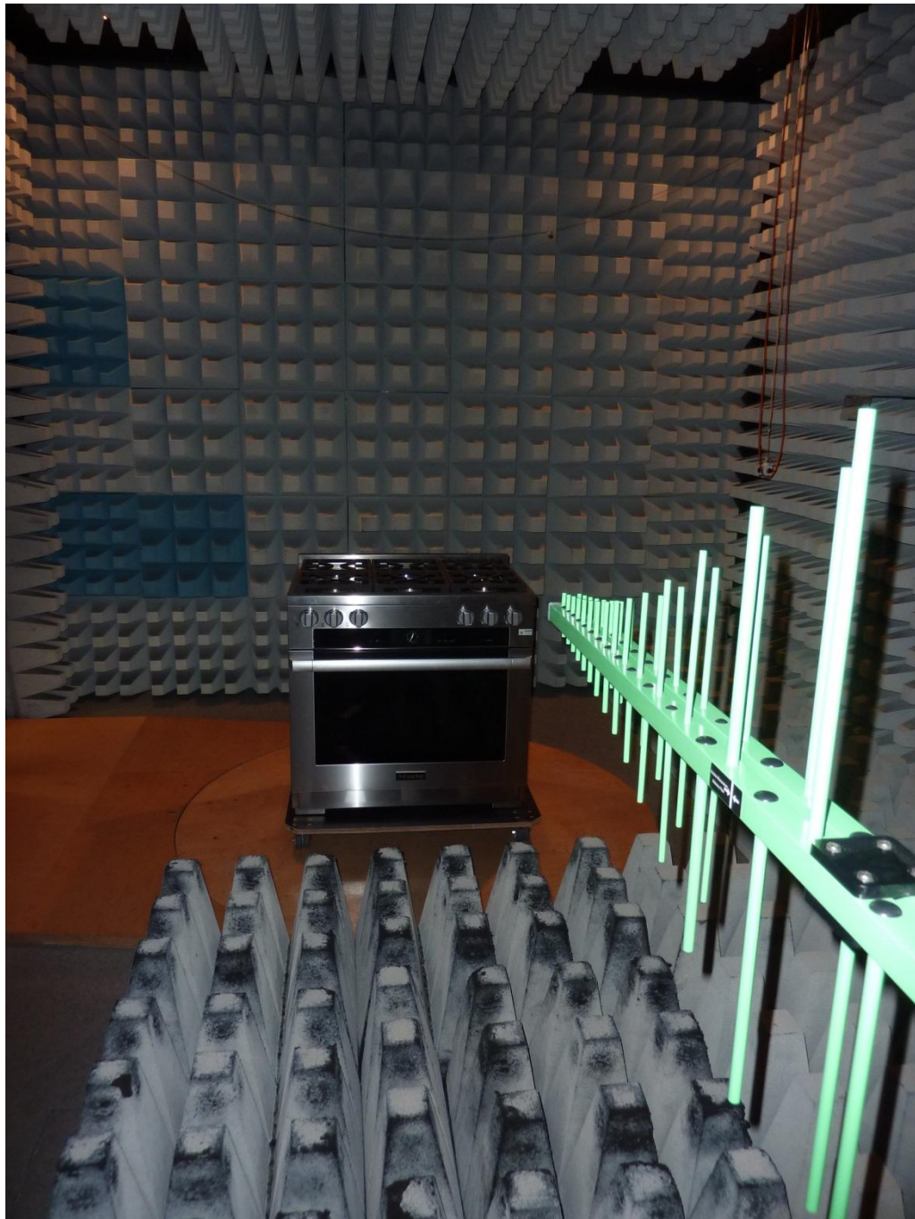
136015_2_1.JPG: EPI7674 inside HR1934, test set-up fully anechoic chamber
