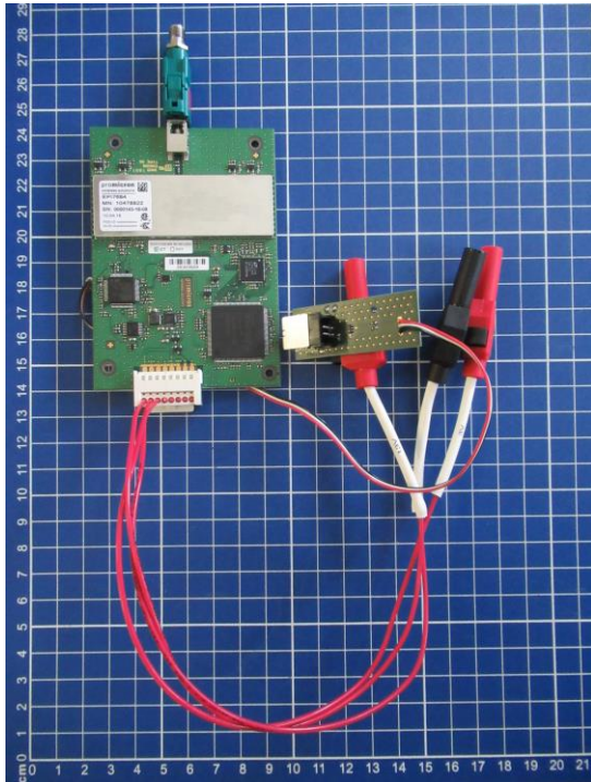
Front view of EUT A EPI7684
