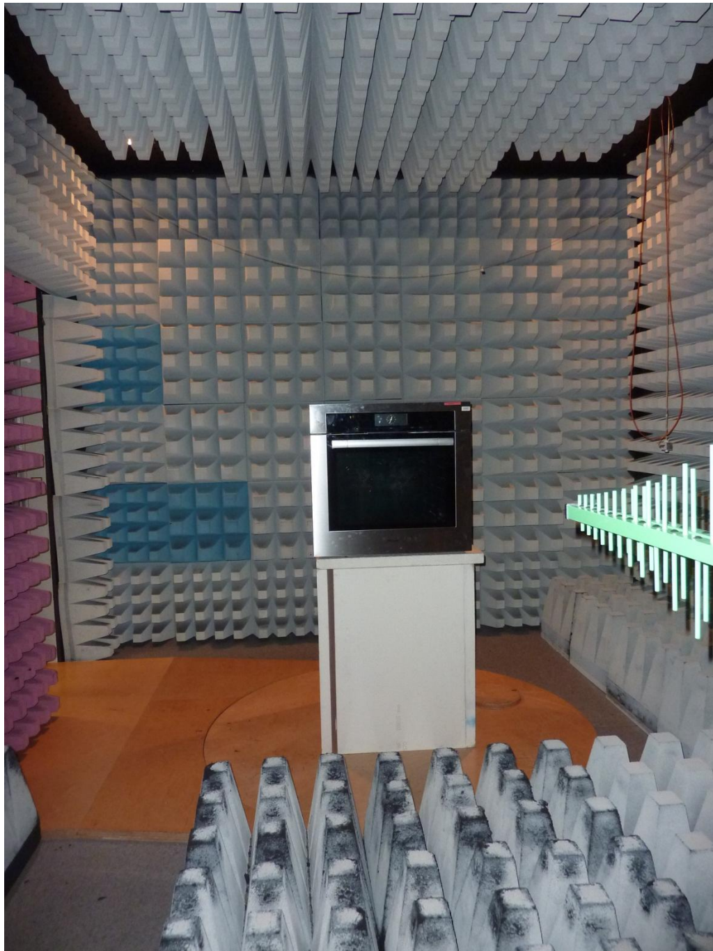
132604_1_1.JPG: EPI7674 inside H6780BP, test set-up fully anechoic chamber
