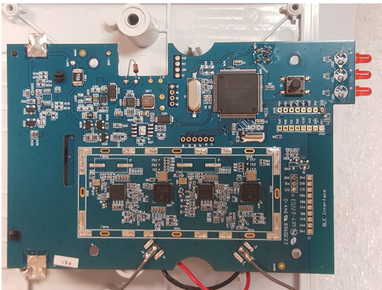
5 PCB Component Side View
