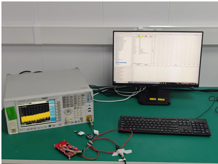
Conducted Test-UHF
