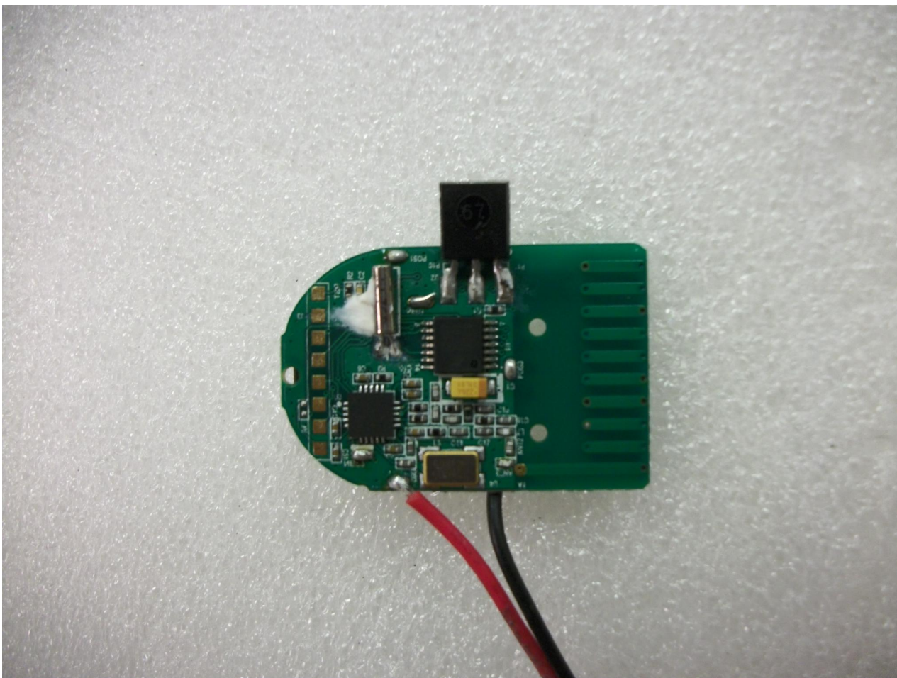
7.3 PCB Component Side View
