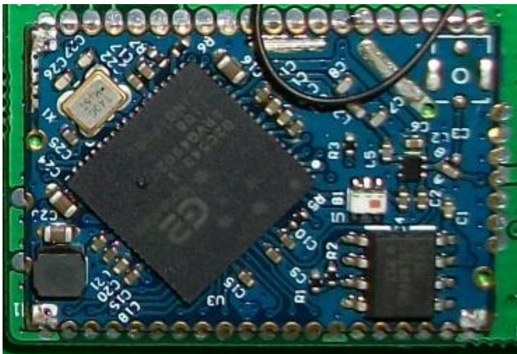
7.7 2.4G Band PCB Open View
