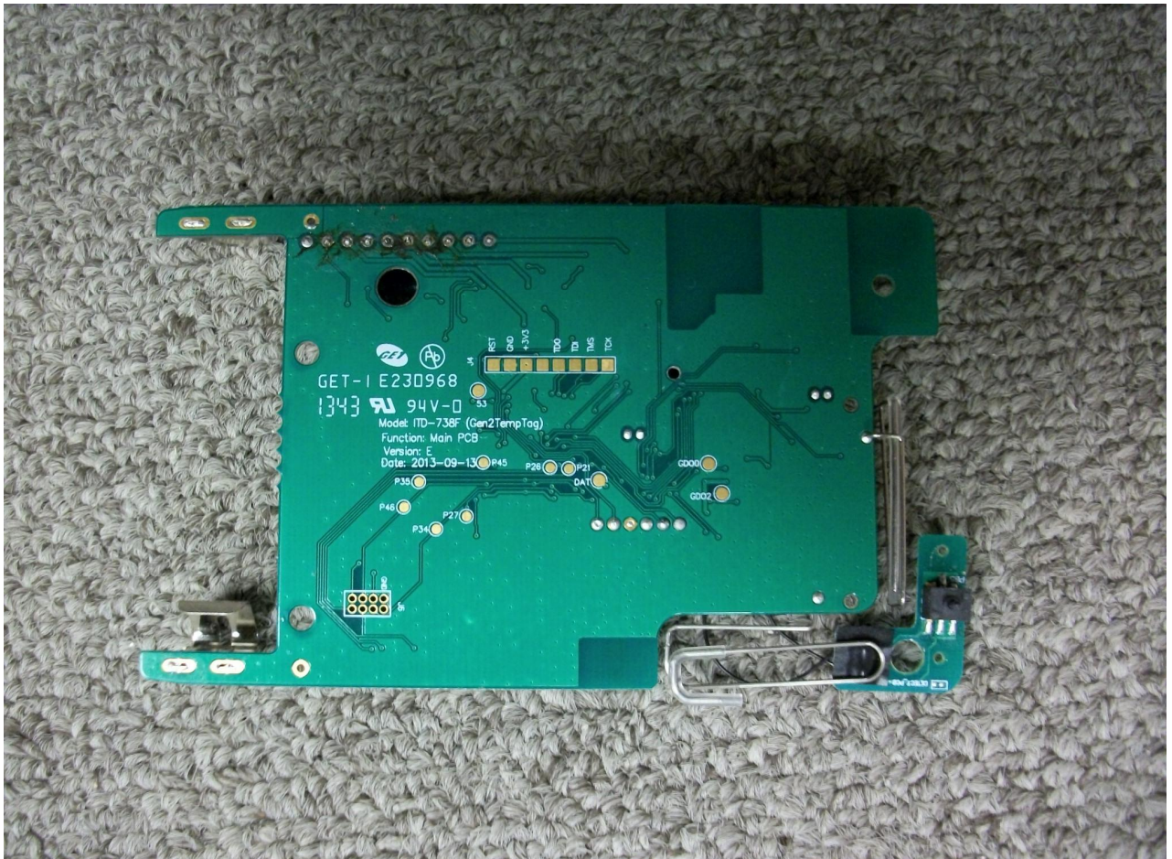
7.6 PCB Foil Side View
