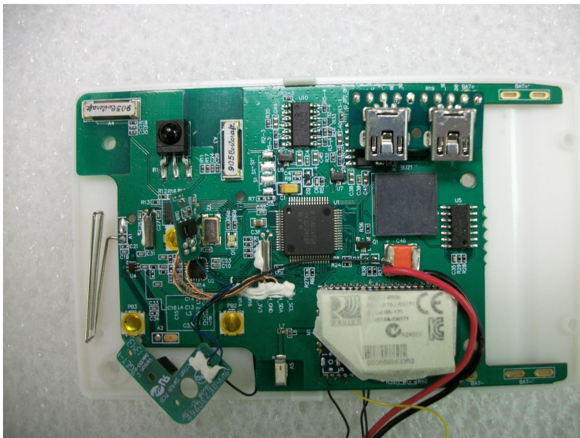
7.5 PCB Component Side View_
