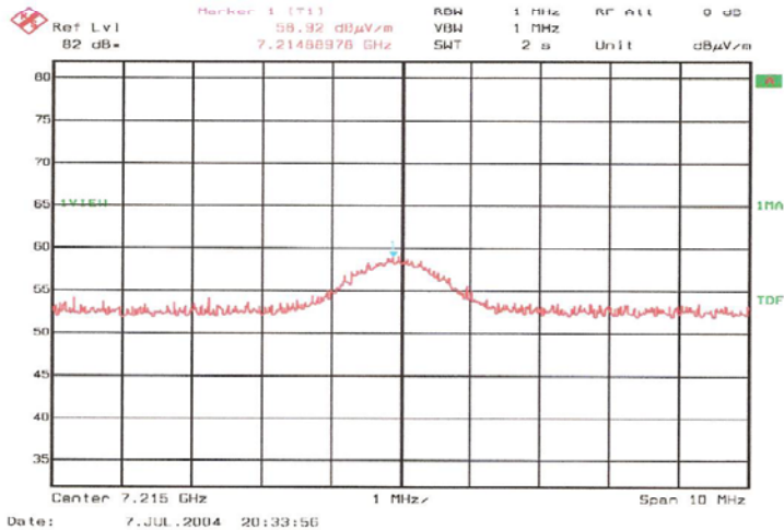
Max field strength –radiated emission, 3 rd Harmonic , ch 11.
