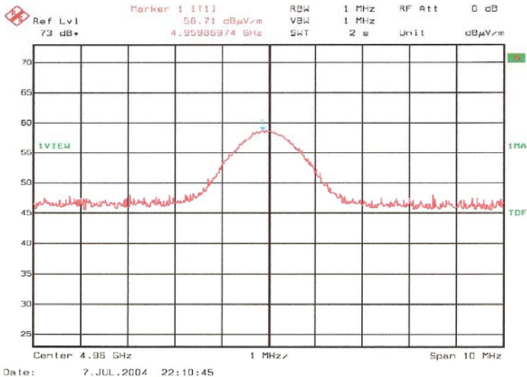
Max field strength –radiated emission, 2 nd Harmonic , ch 26
