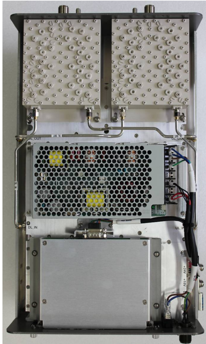
< The Inside of the Repeater >
