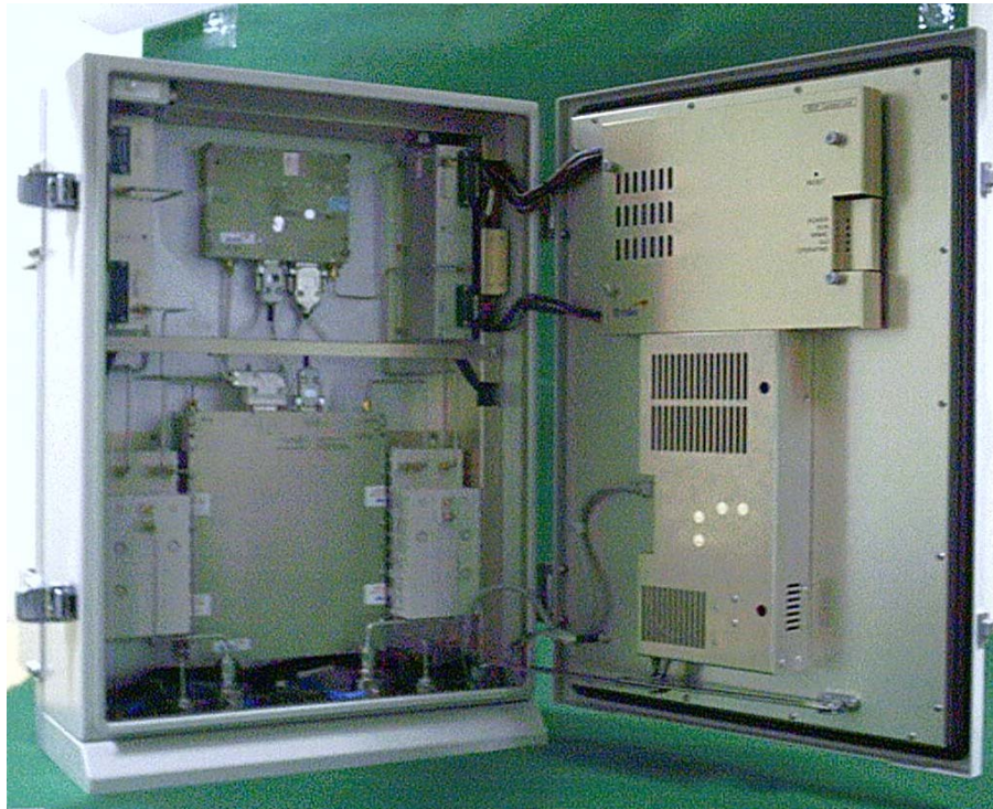
< The Inside of the Repeater >
