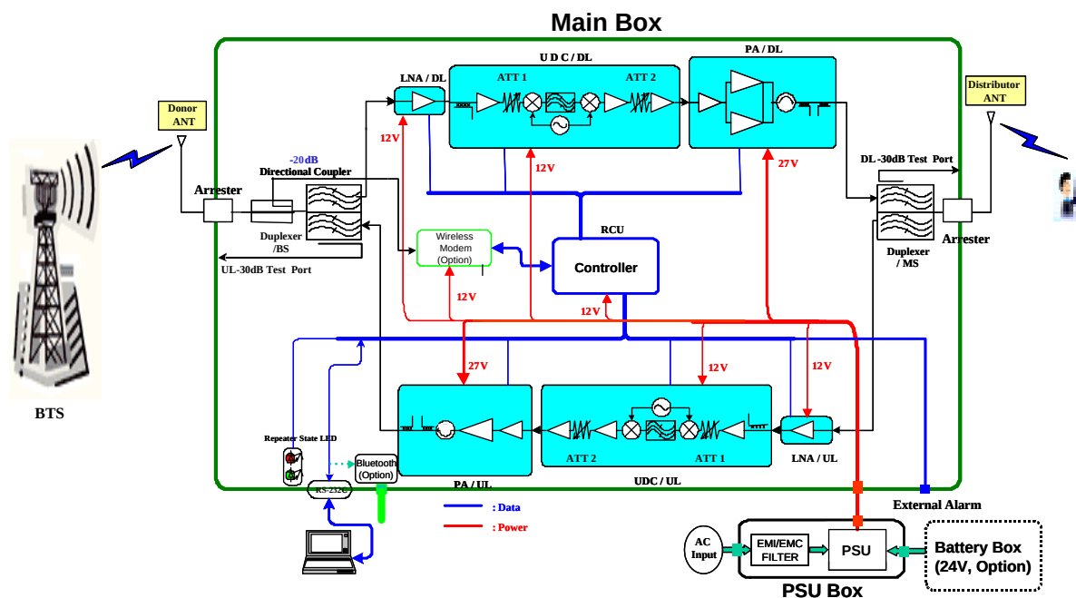
Figure 15 Block Diagram of Band Selective Repeater
