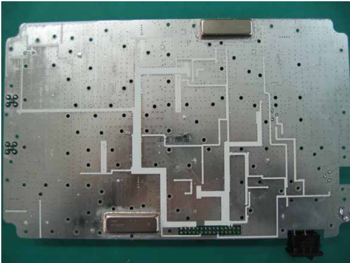
RF PCB 3
