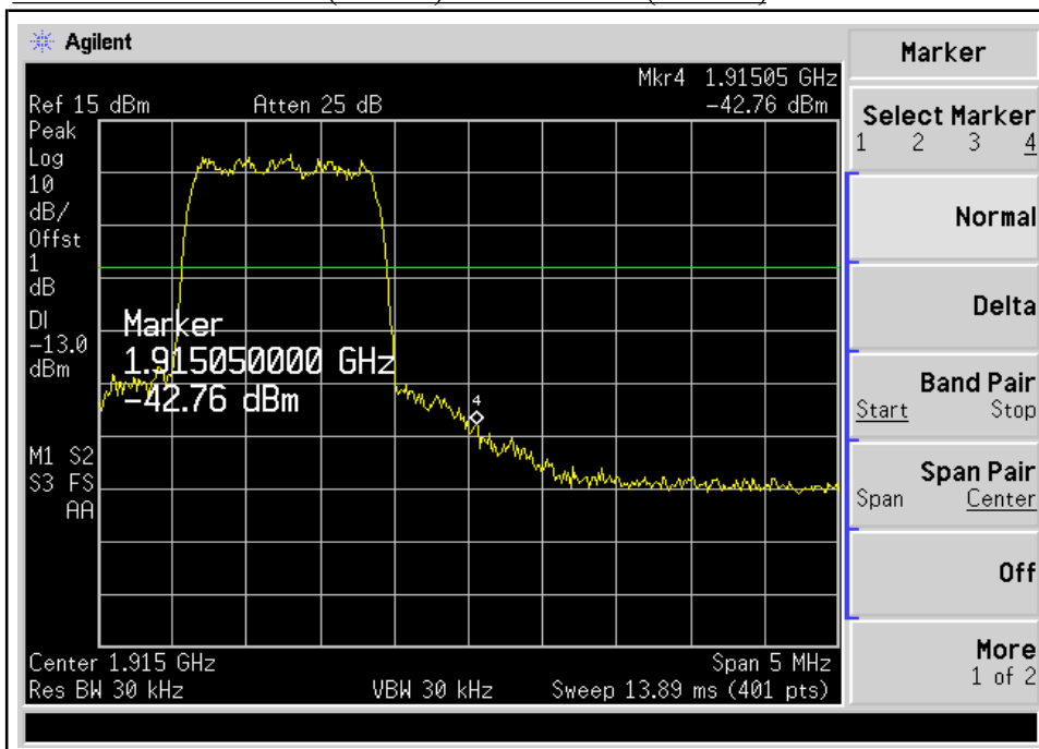
PLOTS OF EMISSION (CDMA): BAND EDGE(Ch1275)
