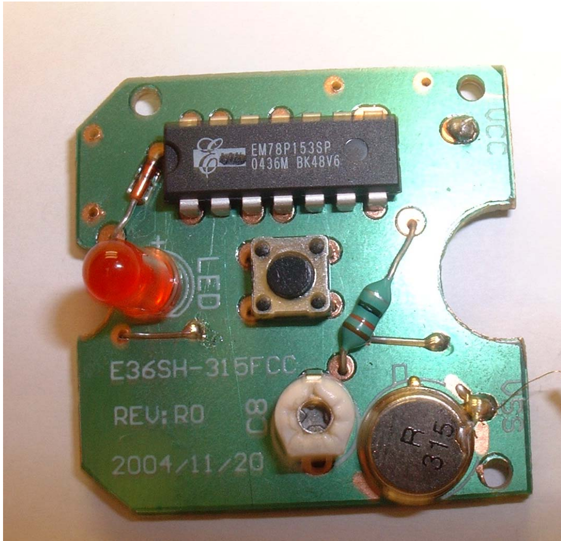
1.11. Figure 11 Transmitter Circuit Board View 2
