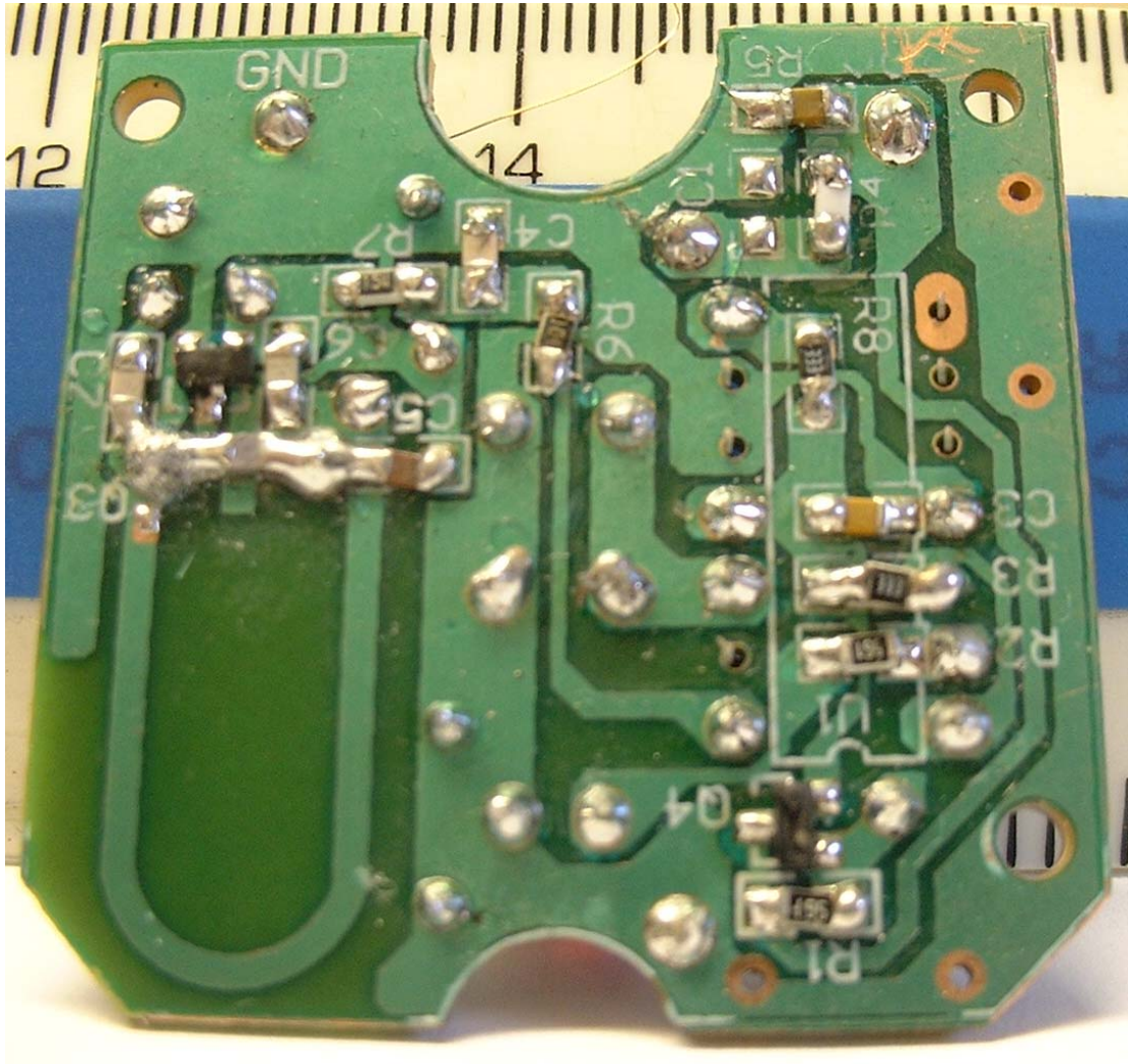
1.8. Figure 8 Transmitter Circuit Board View 1
