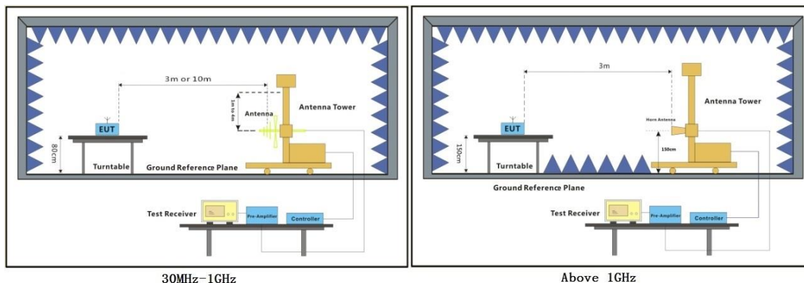
30MHz-1GHz
