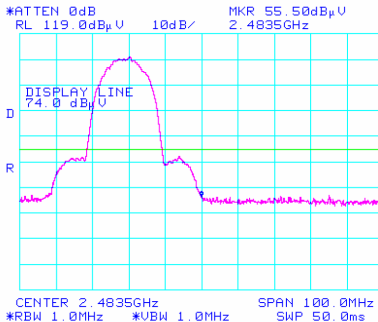
PEAK Limit at Vertical polarization, Upper Edge for 2462 MHz Plot
