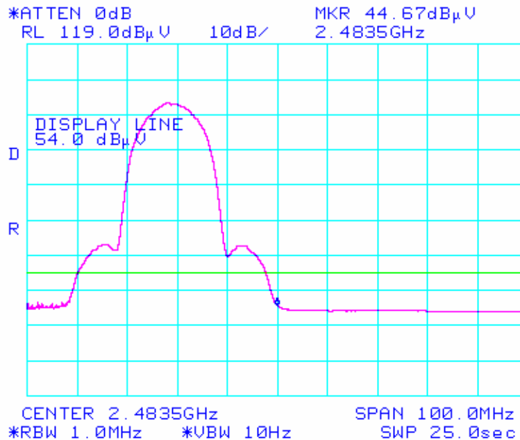
AVERAGE Limit at Vertical polarization, Upper Edge for 2462 MHz Plot
