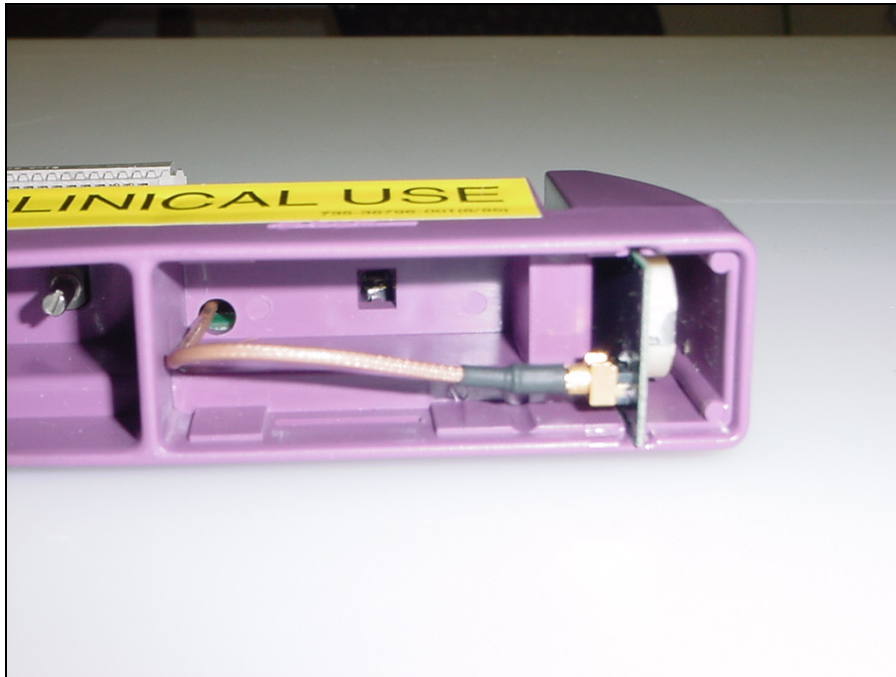
Photograph 5. Antenna mounted in housing
