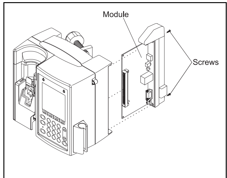
Figure 2. Insert Module
