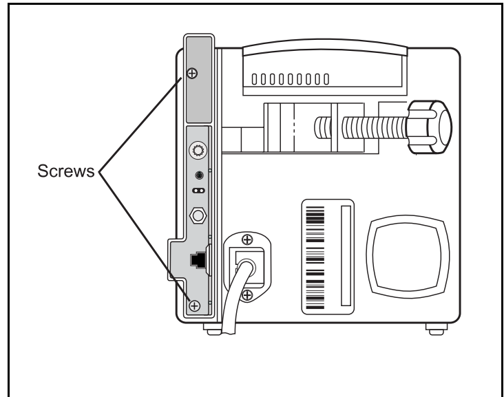
Figure 1. Remove Screws
