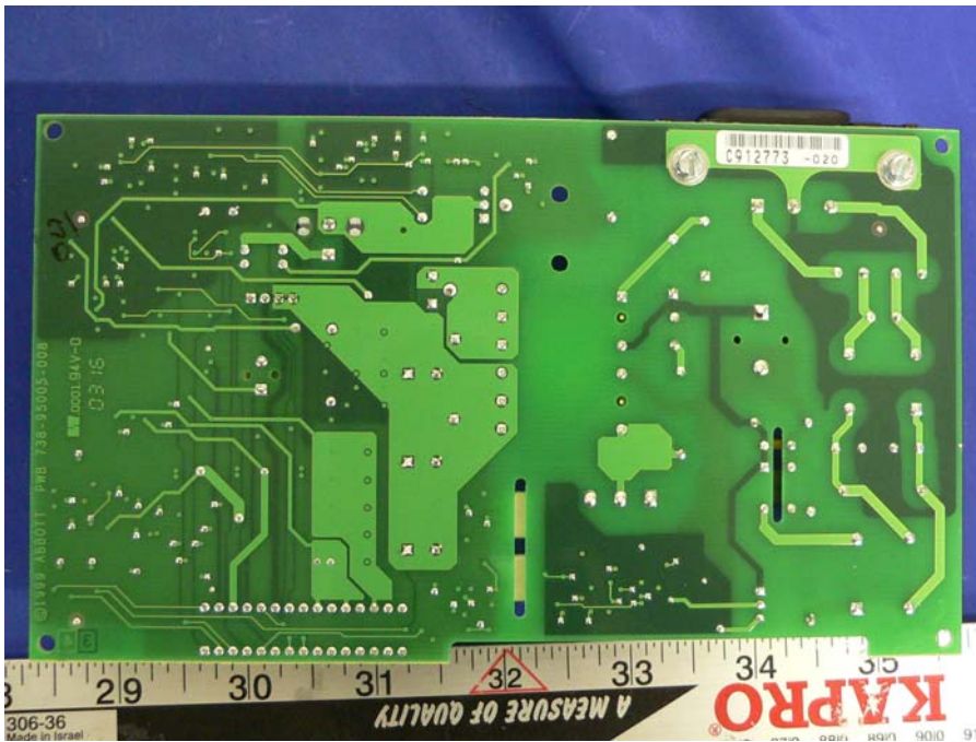
EUT – Power Supply Solder View
