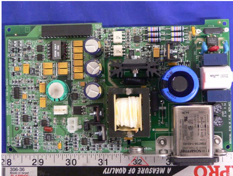
EUT – Power Supply Component View
