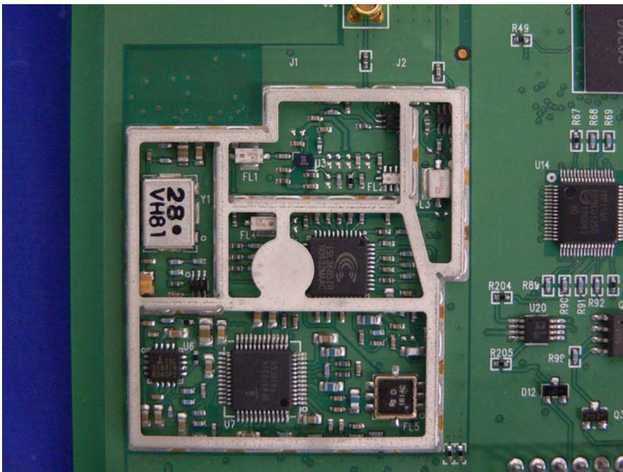
EUT – TX View
