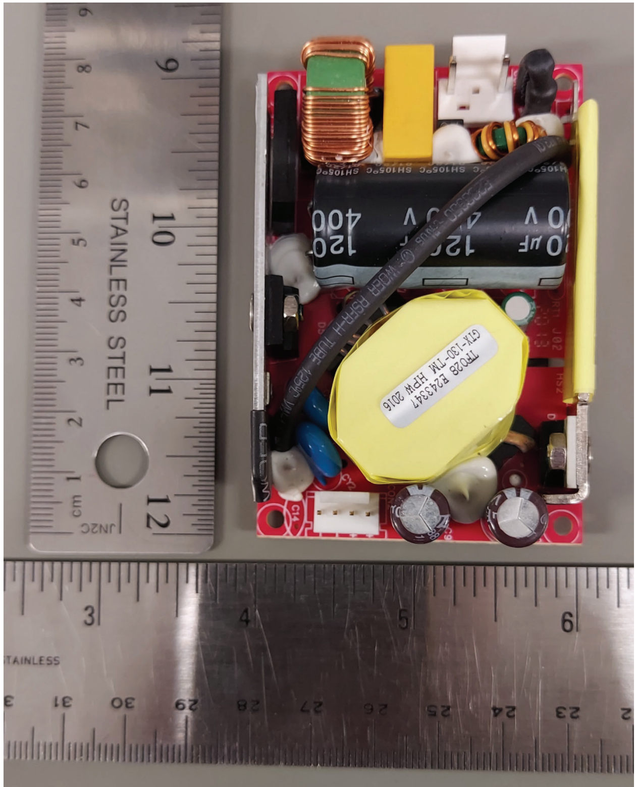
Power Board
