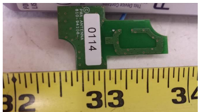
Antenna Bottom View
