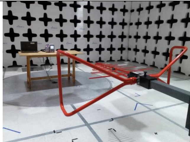
Test setup (<1GHz) - Front
