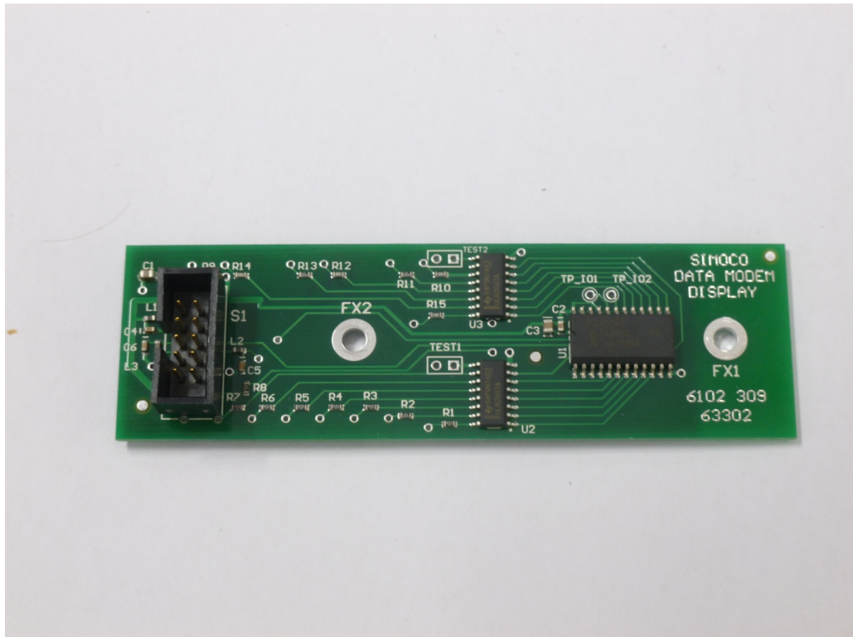
Data modem LED display board top
