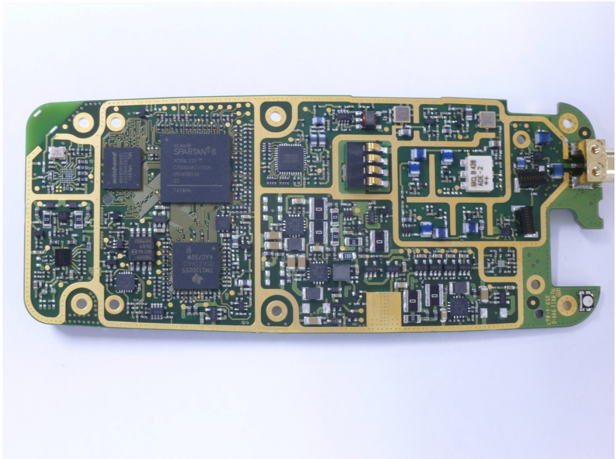
Data Modem SDD690 AC Engine PCB top
