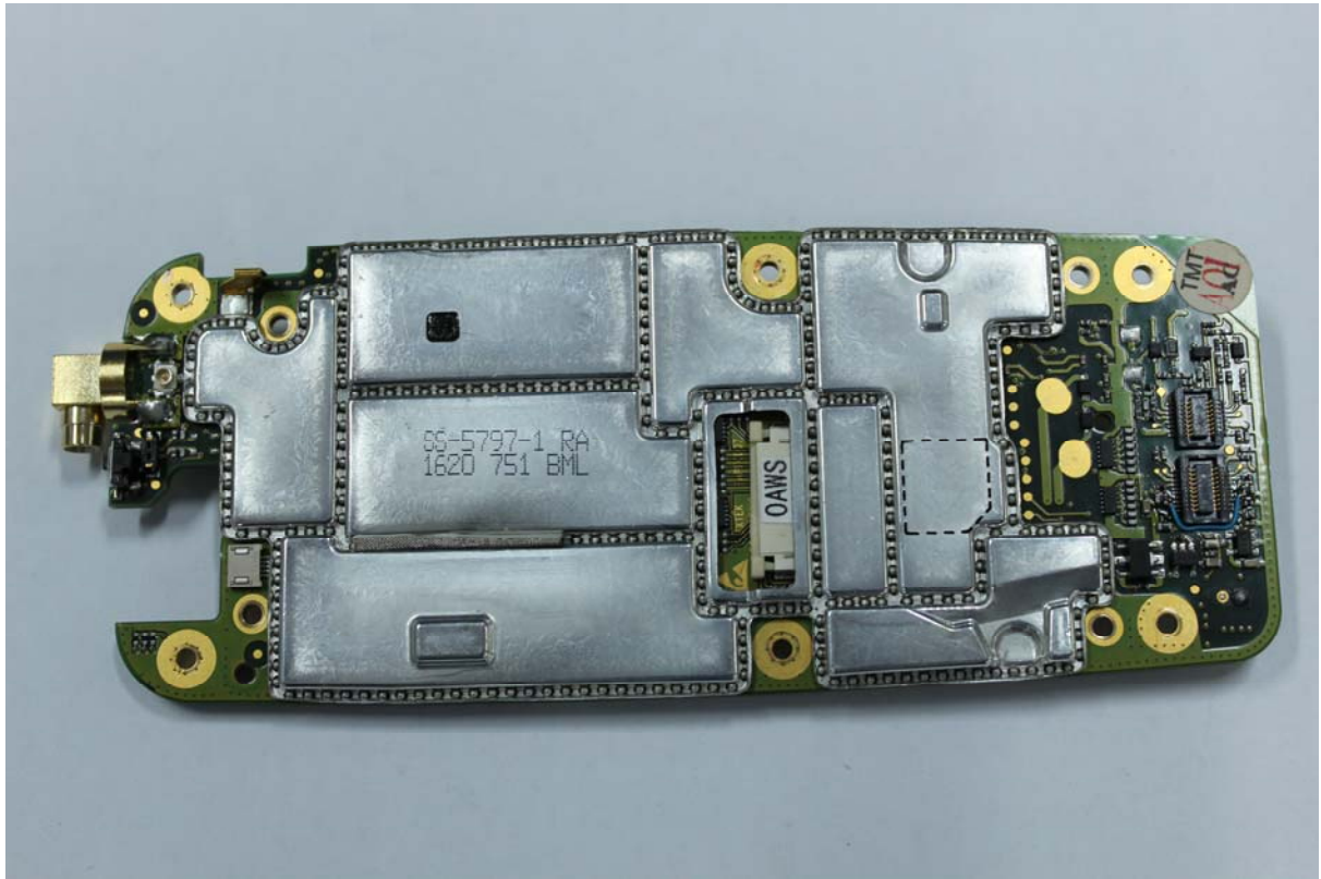
Data Modem SDD690 AC Engine PCB bottom with shield
