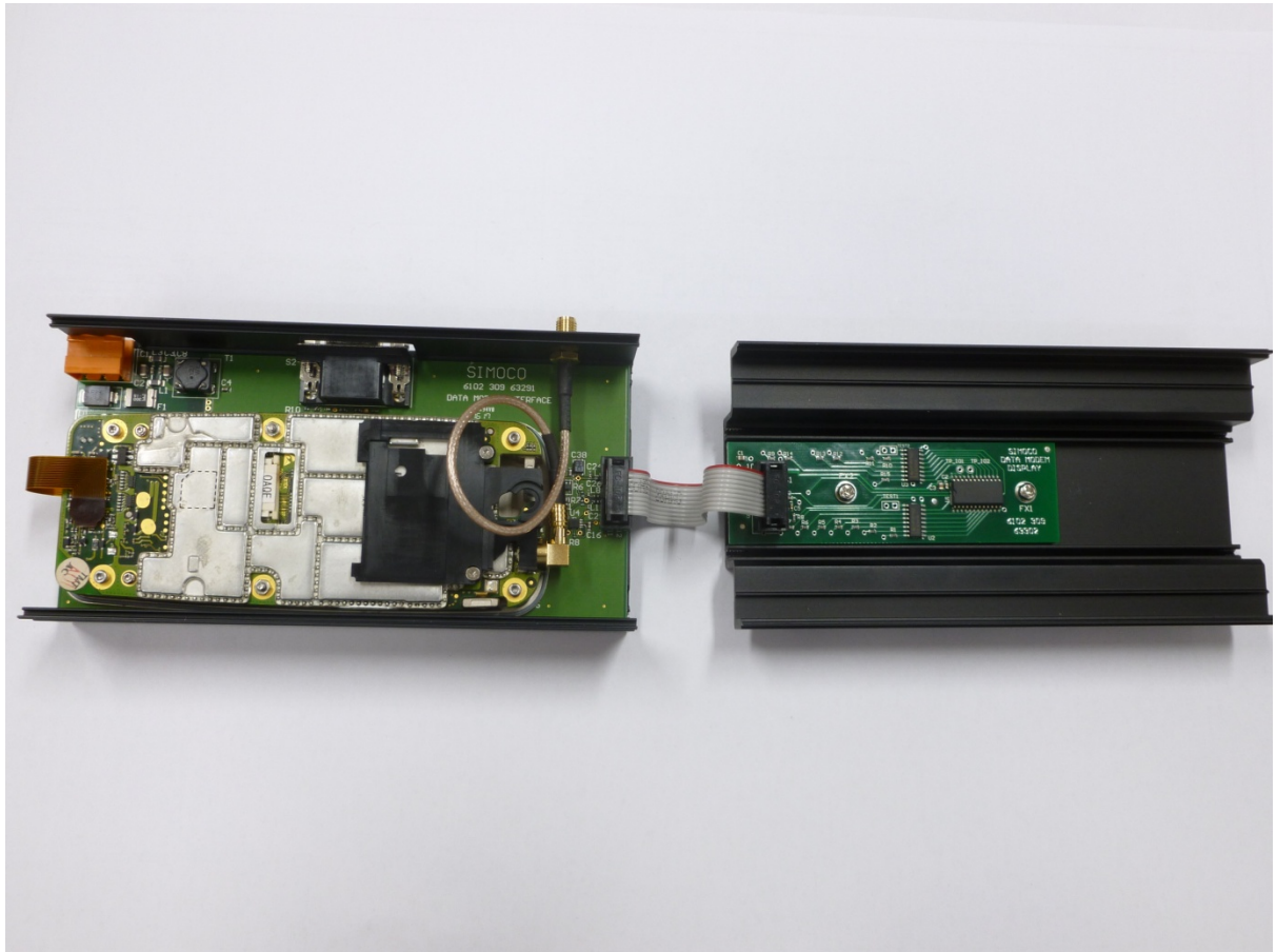
Data modem open enclosure
