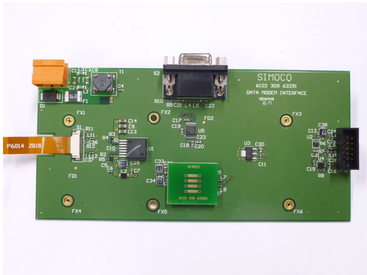
Data Modem Serial Interface board top
