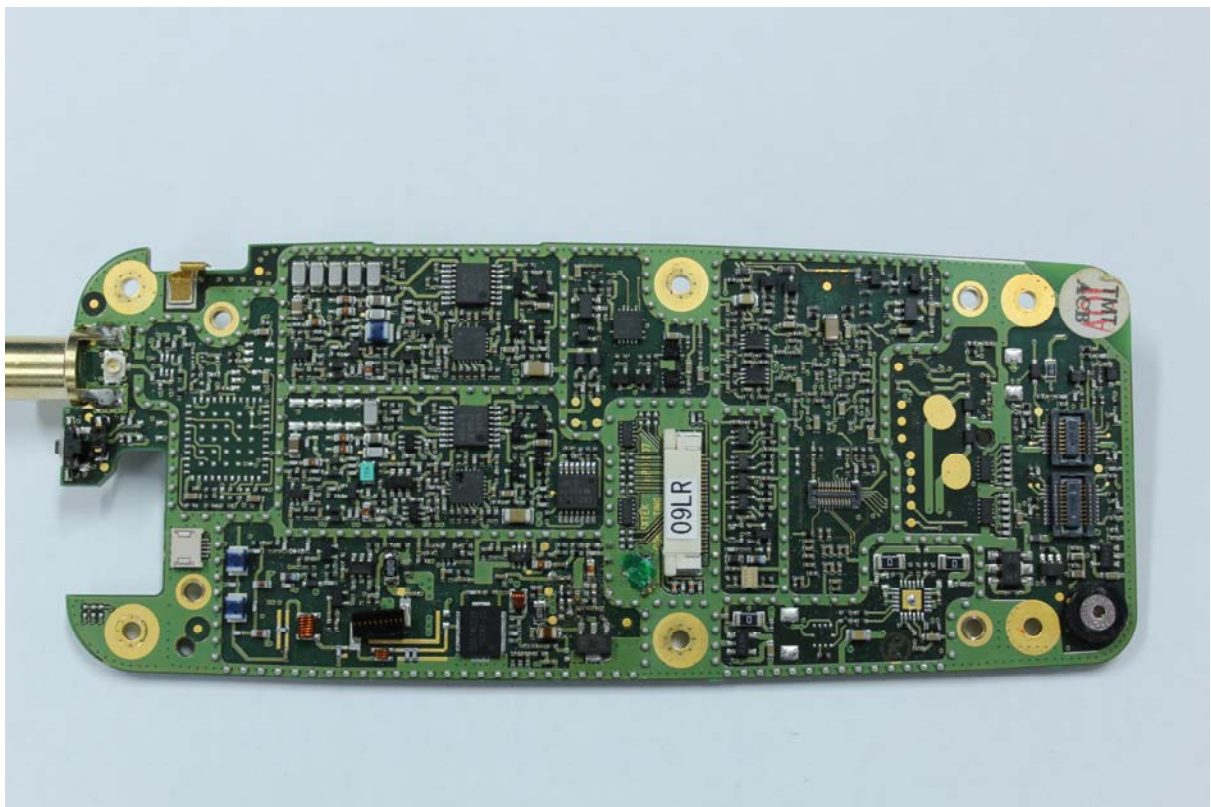
Data Modem SDD690 AC Engine PCB bottom with no shield (a 2nd attempt)
