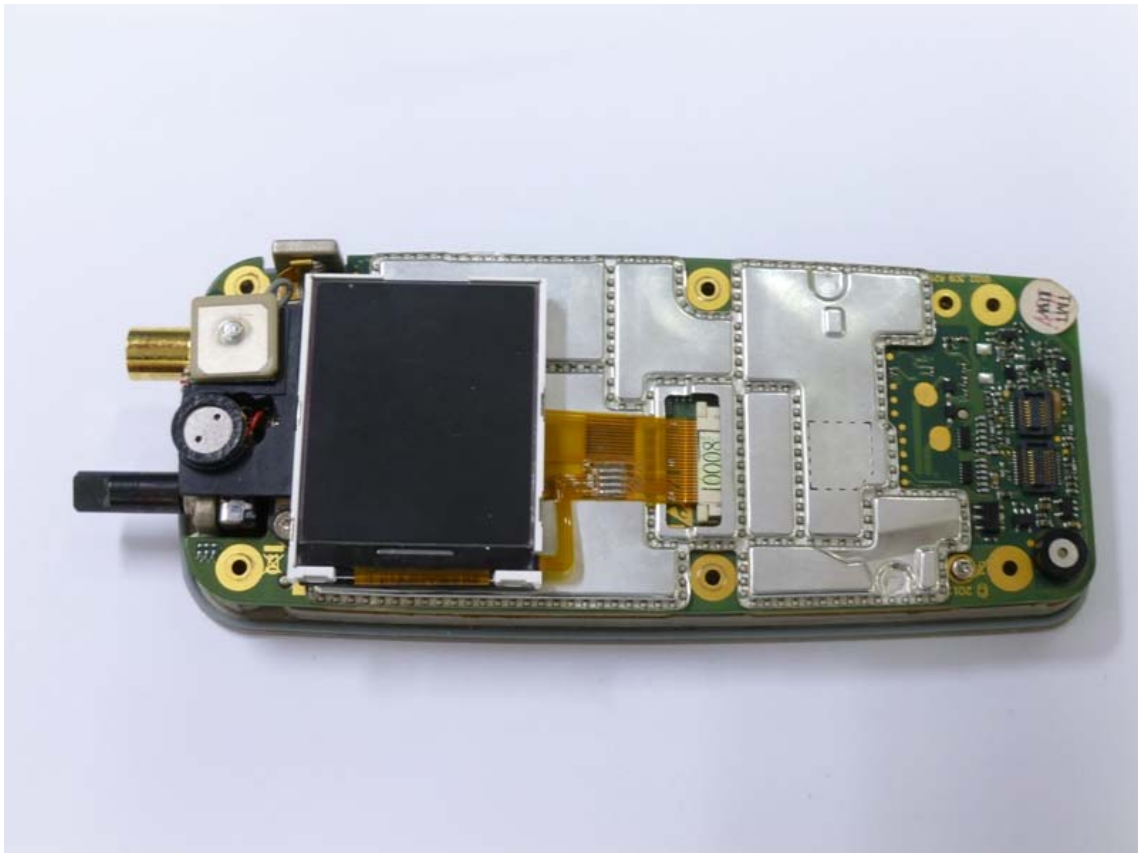
SDP600UW Bottom with LCD
