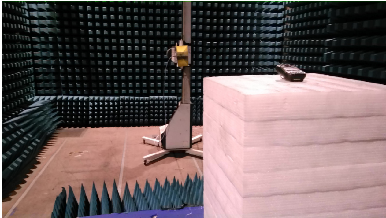
Above 1GHz
