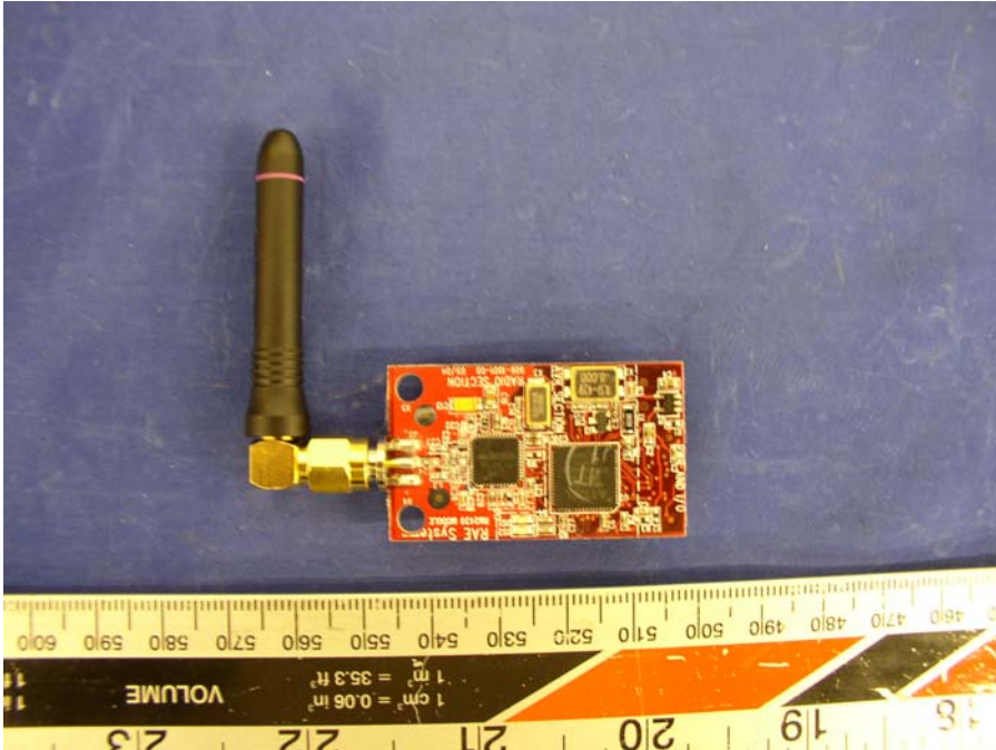
EUT – Cover Removed Top View
