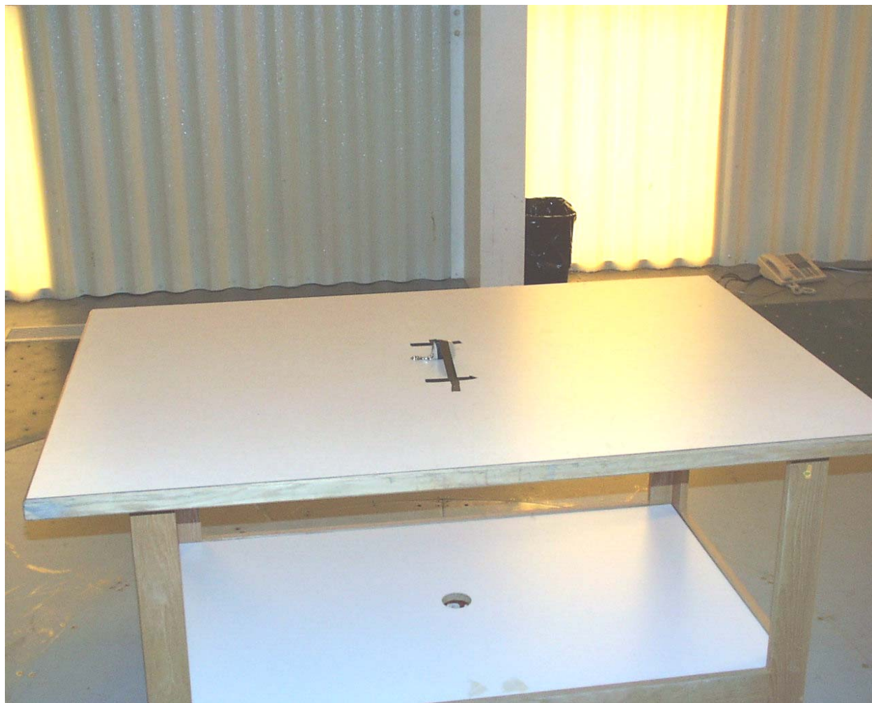
Photograph 2 - View of the Radiated Emission Test Setup (Horizontal Face Alignment)
