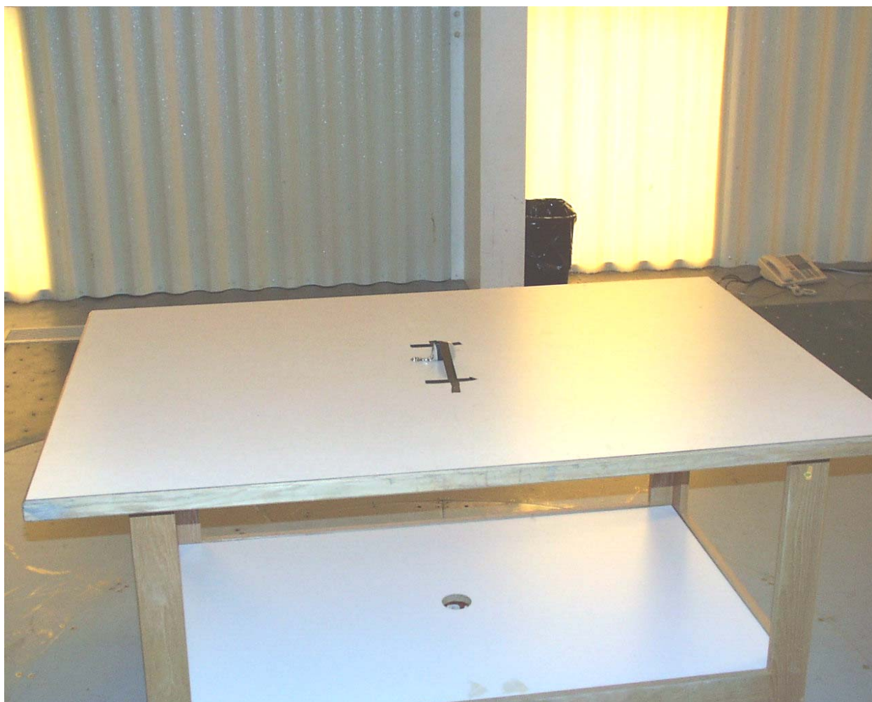
View of the Radiated Emission Test Setup (Horizontal Face Alignment)
