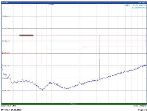
Figure 8.4-1: Horizontal polarization, Radiated spurious emissions below 1 GHz, E.U.T in horizontal position
