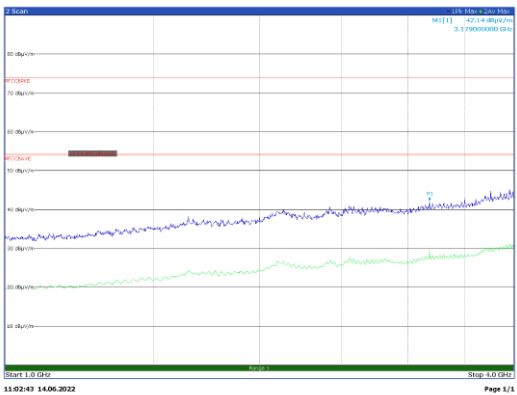
Figure 8.4-8: Vertical polarization, Radiated spurious emissions above 1 GHz, E.U.T in vertical position
