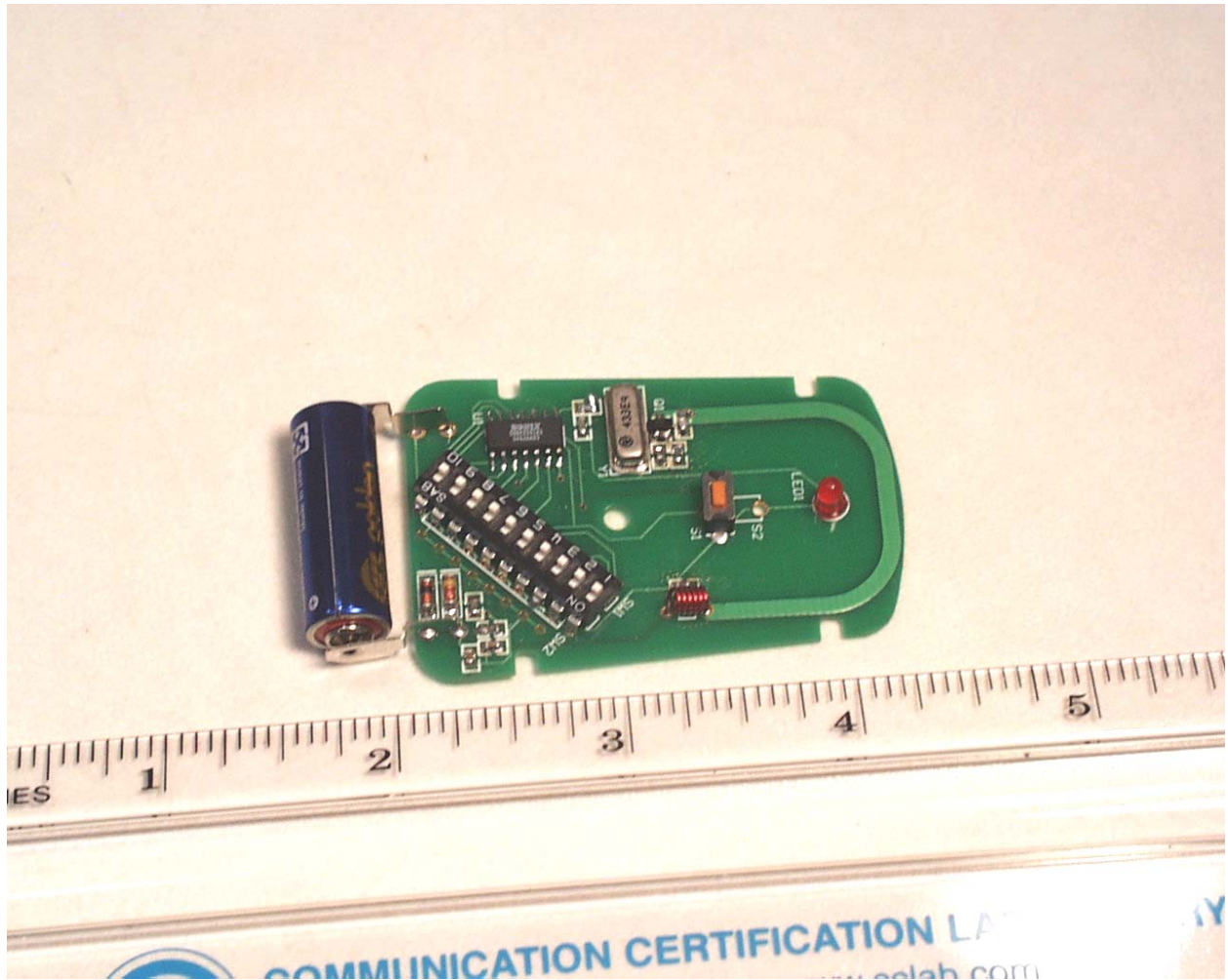
Photograph 6 - View of the Component Side of the PCB
