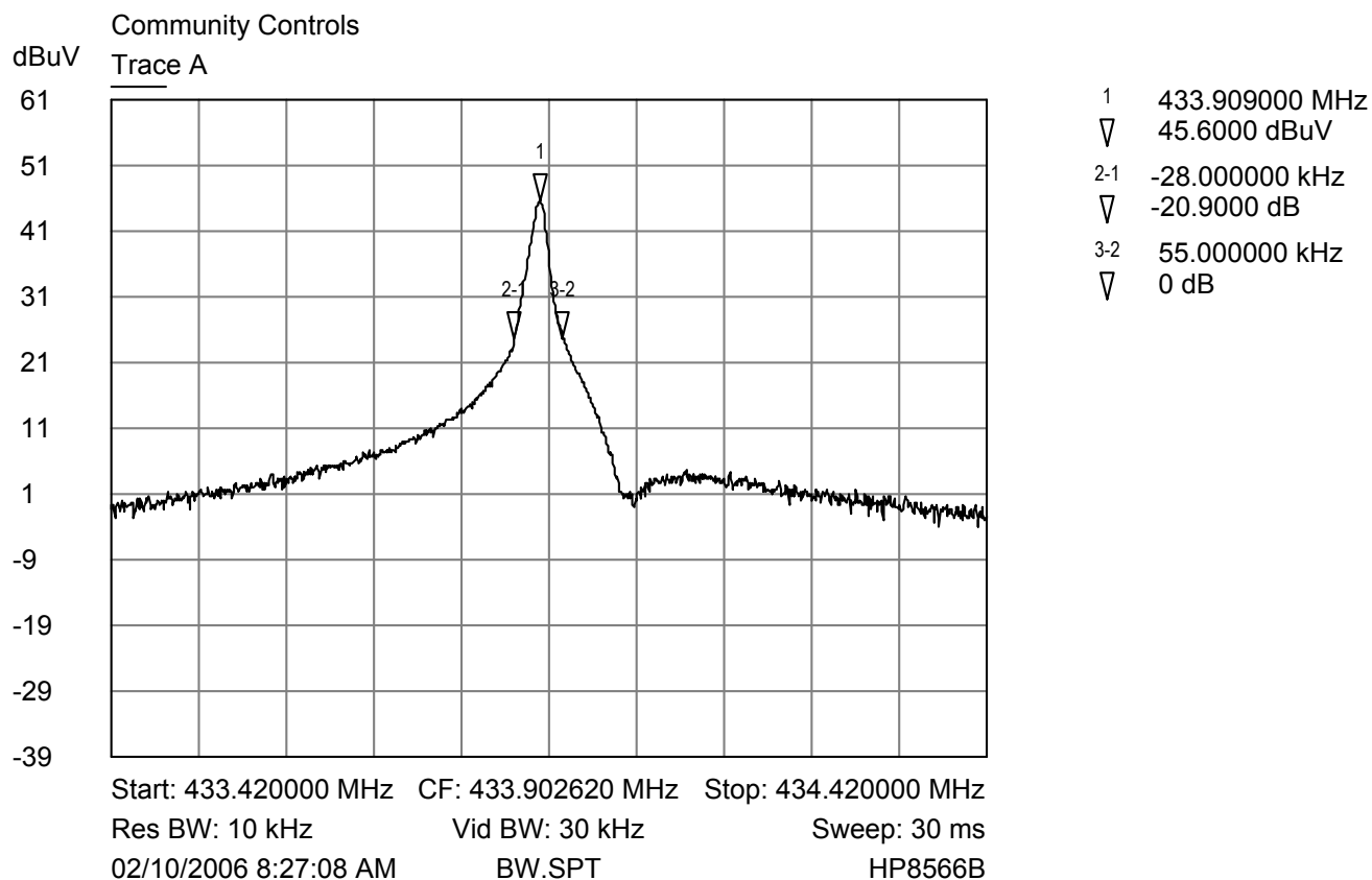
Bandwidth Plot
