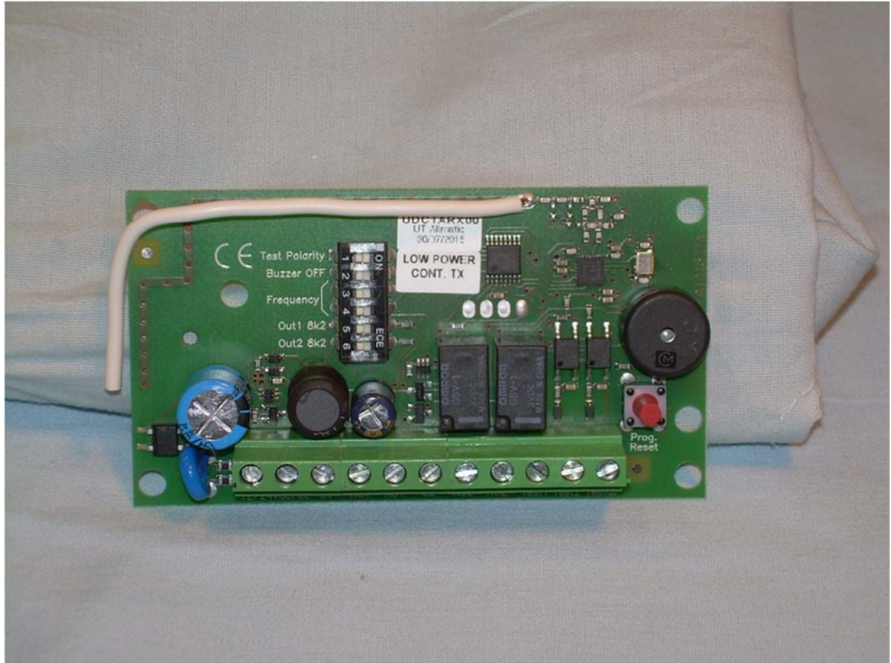
View of the Component Side of the RCO0900
