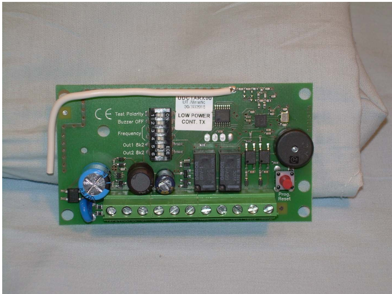
Photograph 8 – View of the Component Side of the RCOO900
