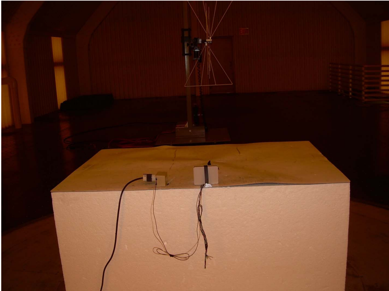
Photograph 2 – Back View Radiated Test Setup – RCO0900
