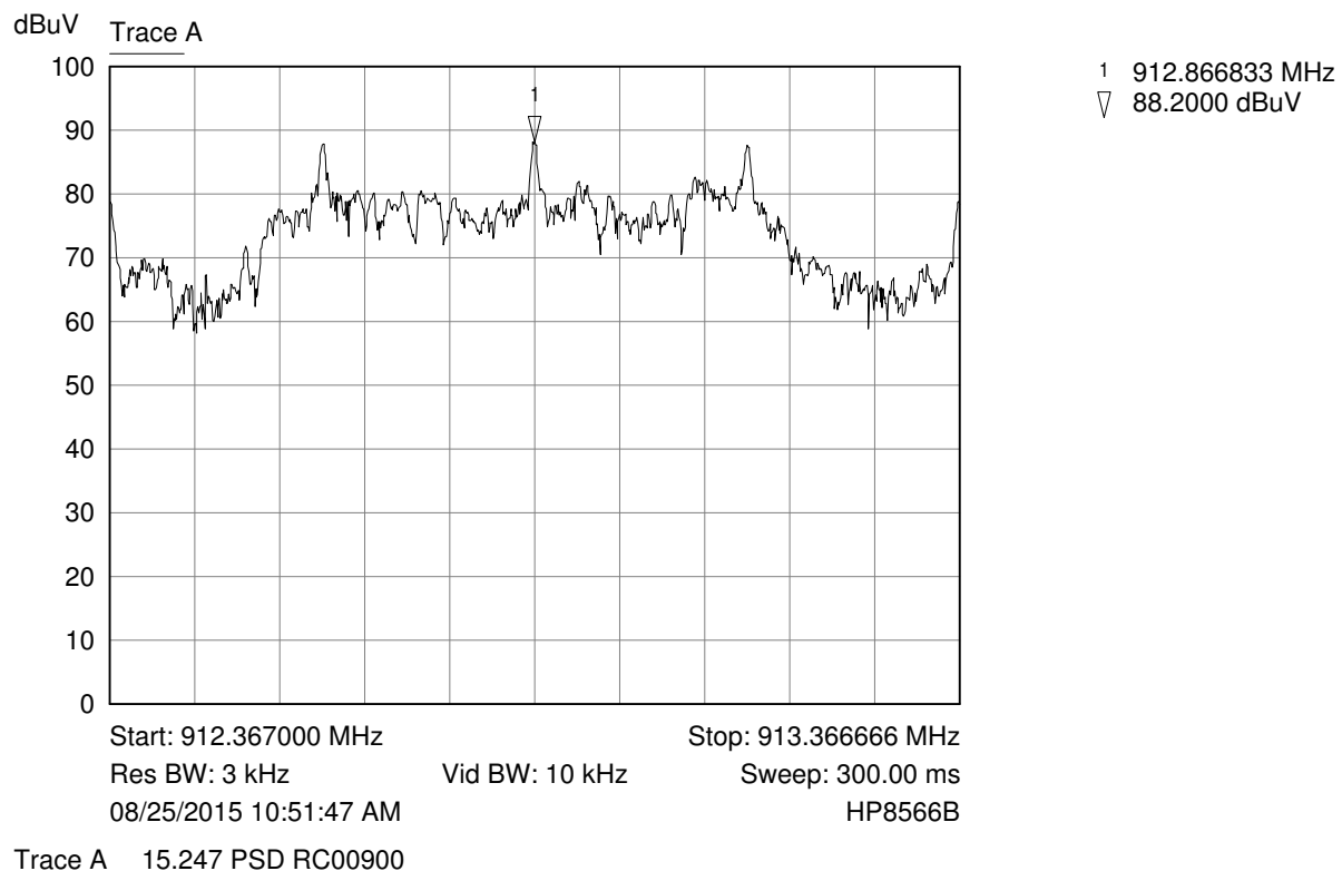
Lowest Channel 3 kHz PSD Plot
