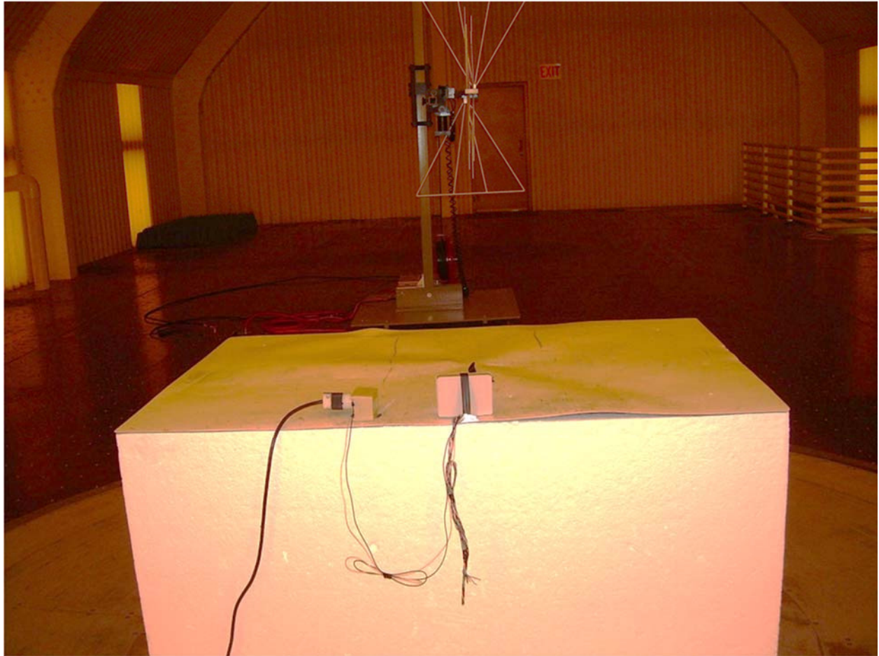
Back View Radiated Test Setup – RCOO900
