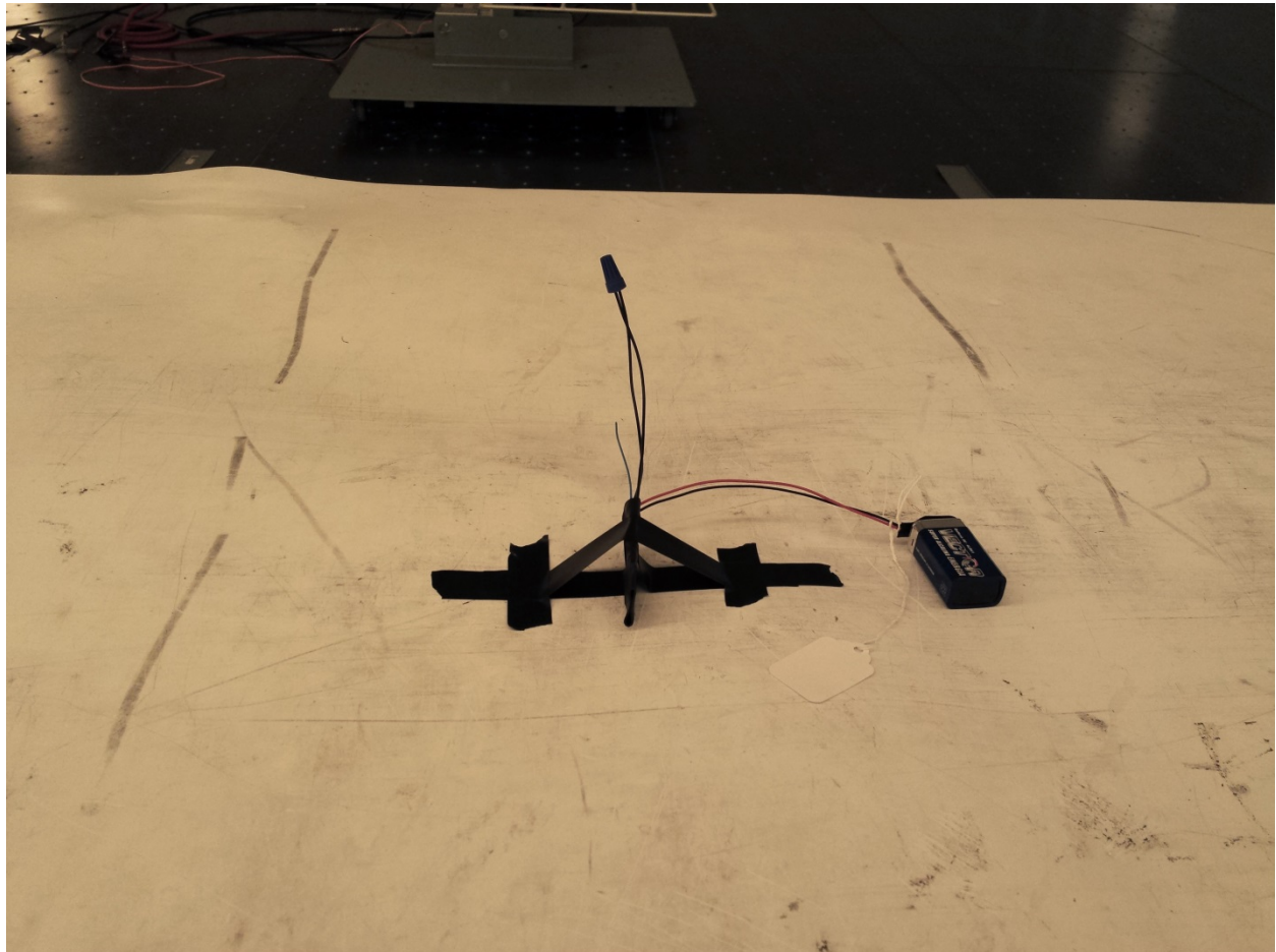
Photograph 3 – Radiated Disturbance – On-edge Configuration
