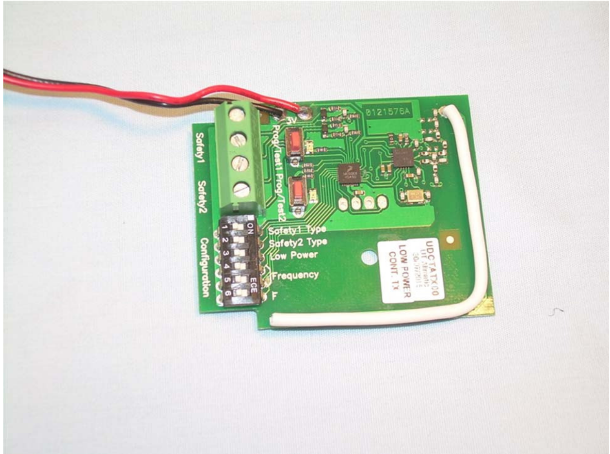
View of the Component Side of the TCOO900
