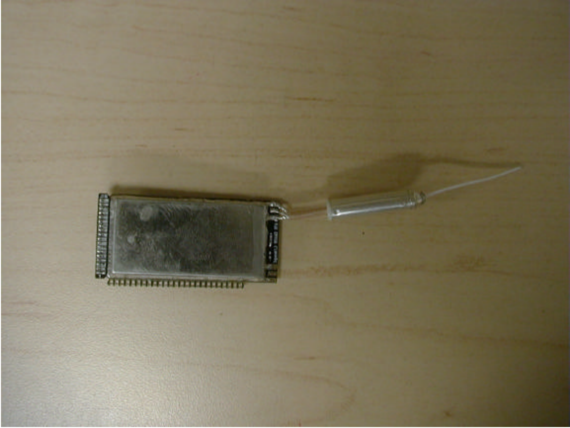
BACK W/ SHIELD ANTENNA SOLDERED ON.
