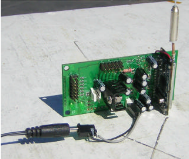
RF section onto Audio/Voltage regulator board
