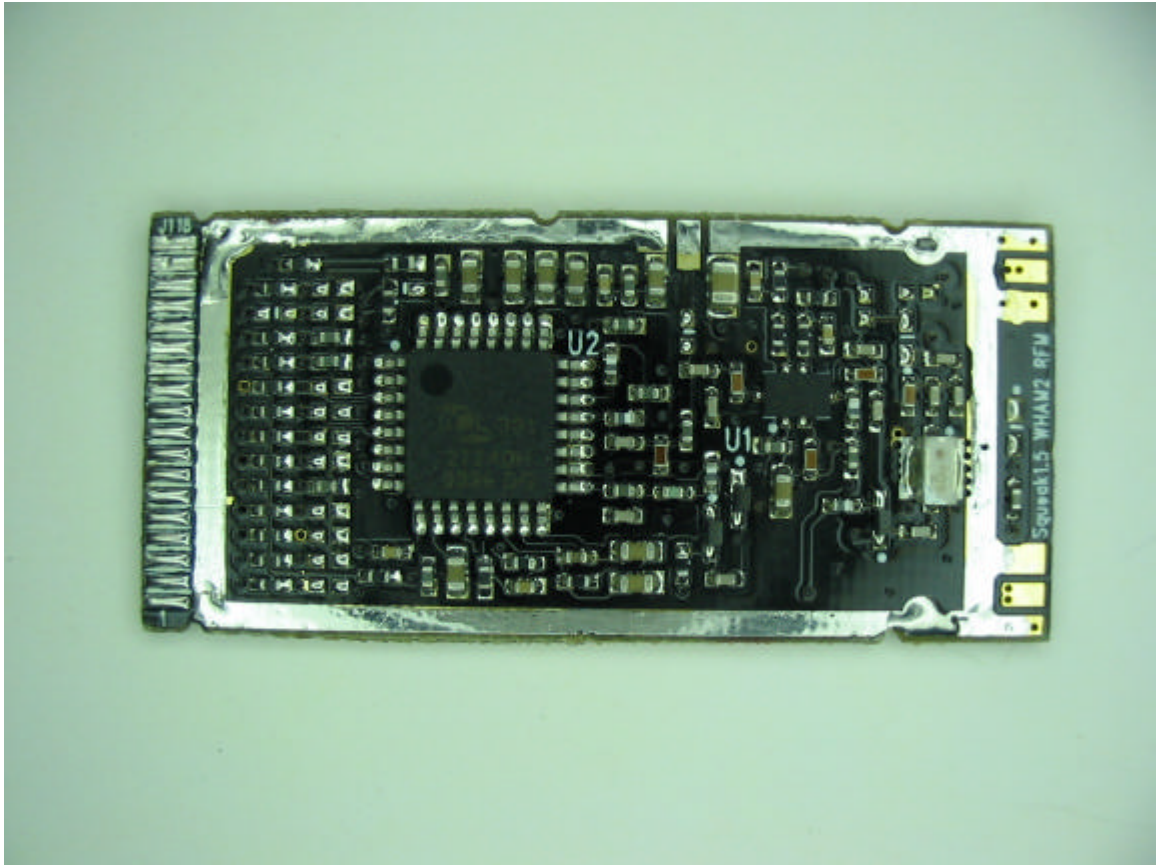
BACK W/O SHIELD
