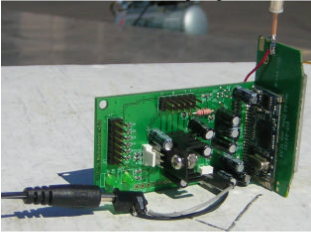
RF section onto Audio/Voltage regulator board
