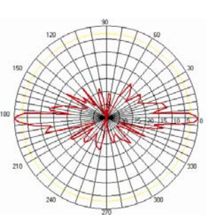
OD9-11D1 E Plane
