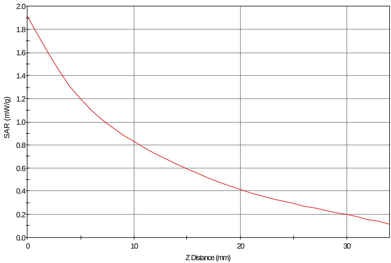
SAR - Z Axis at Hotspot x:-15.0 y:36.0
