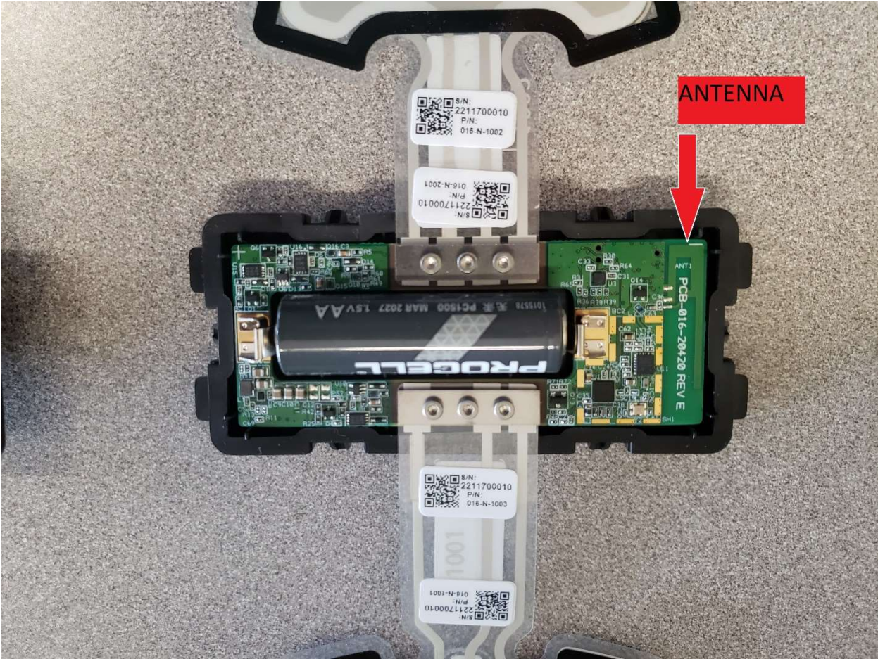
Top Side, Antenna View
