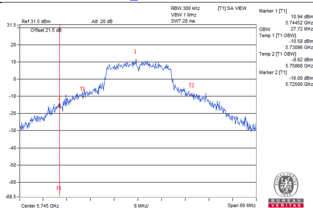
802.11ac(VHT20)_Chain1 / CH149
