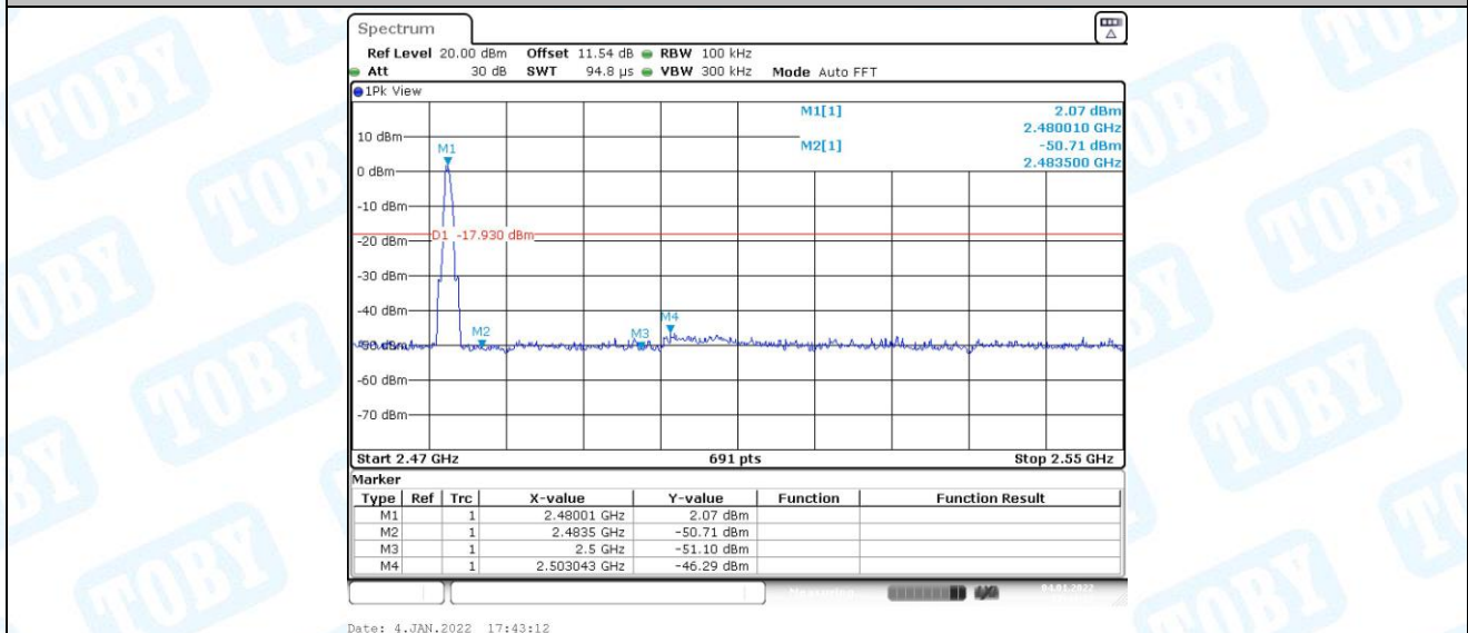
BLE_1M_Ant1_High_2480
