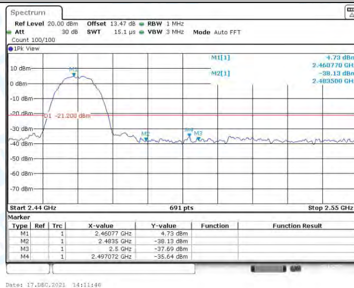
11B-CDD_Ant1_High_2462_Peak
