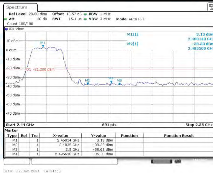
11G-CDD_Ant2_High_2462_Peak
