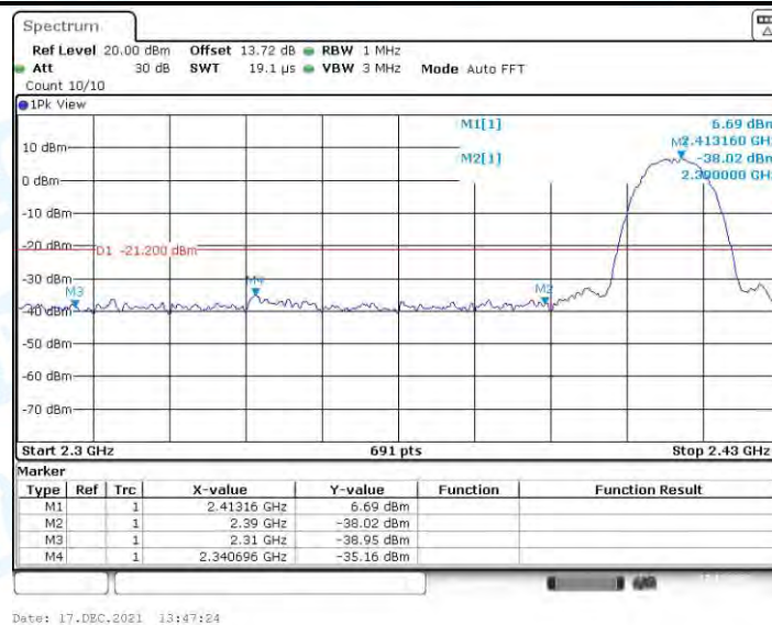
11B-CDD_Ant2_Low_2412_Peak
