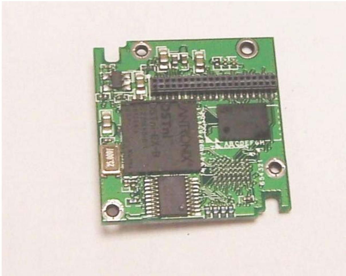
Fig. 10 RF module – lower pcb – bottom view
