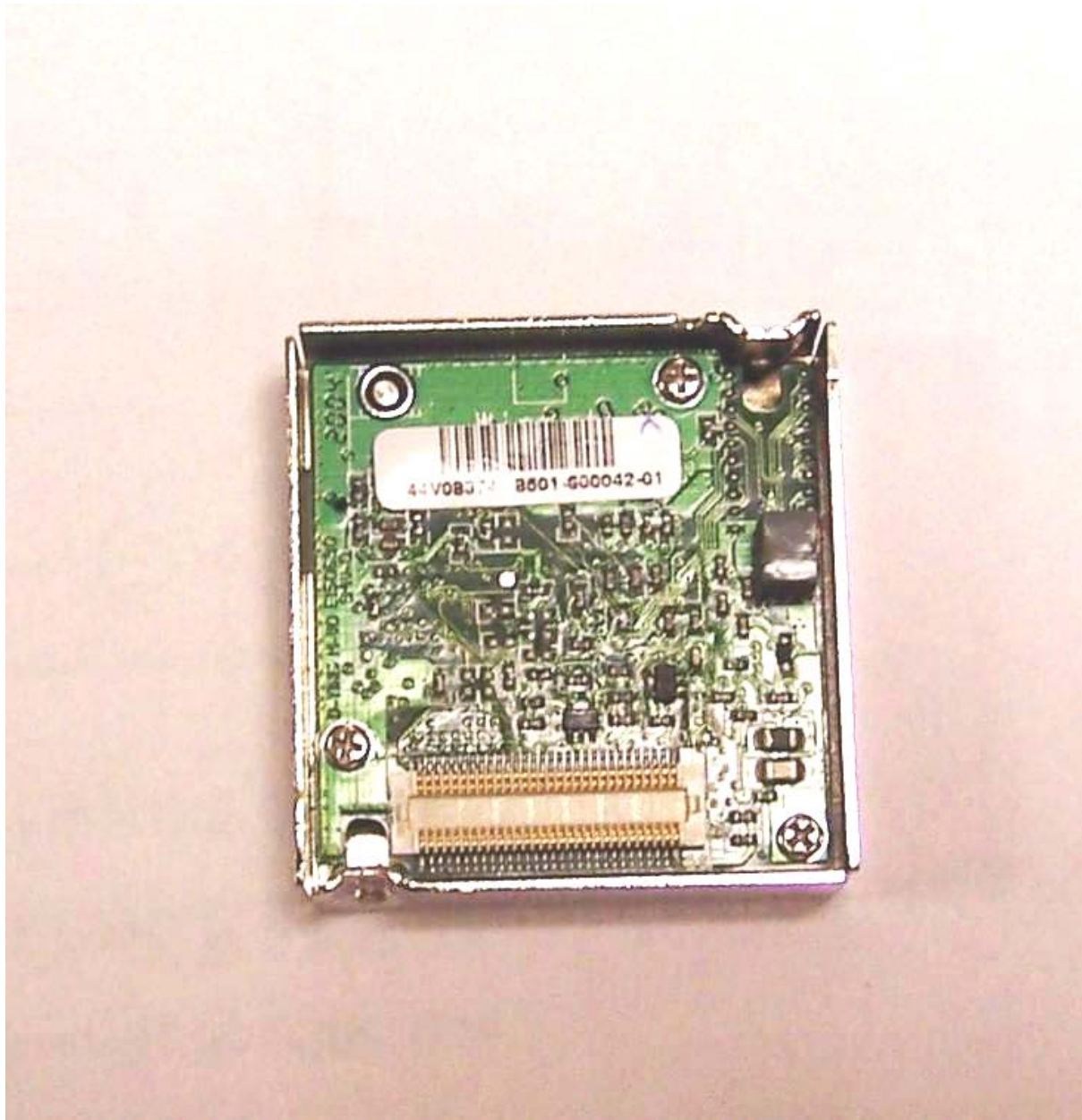
Fig. 9 RF module – lower pcb – top view
