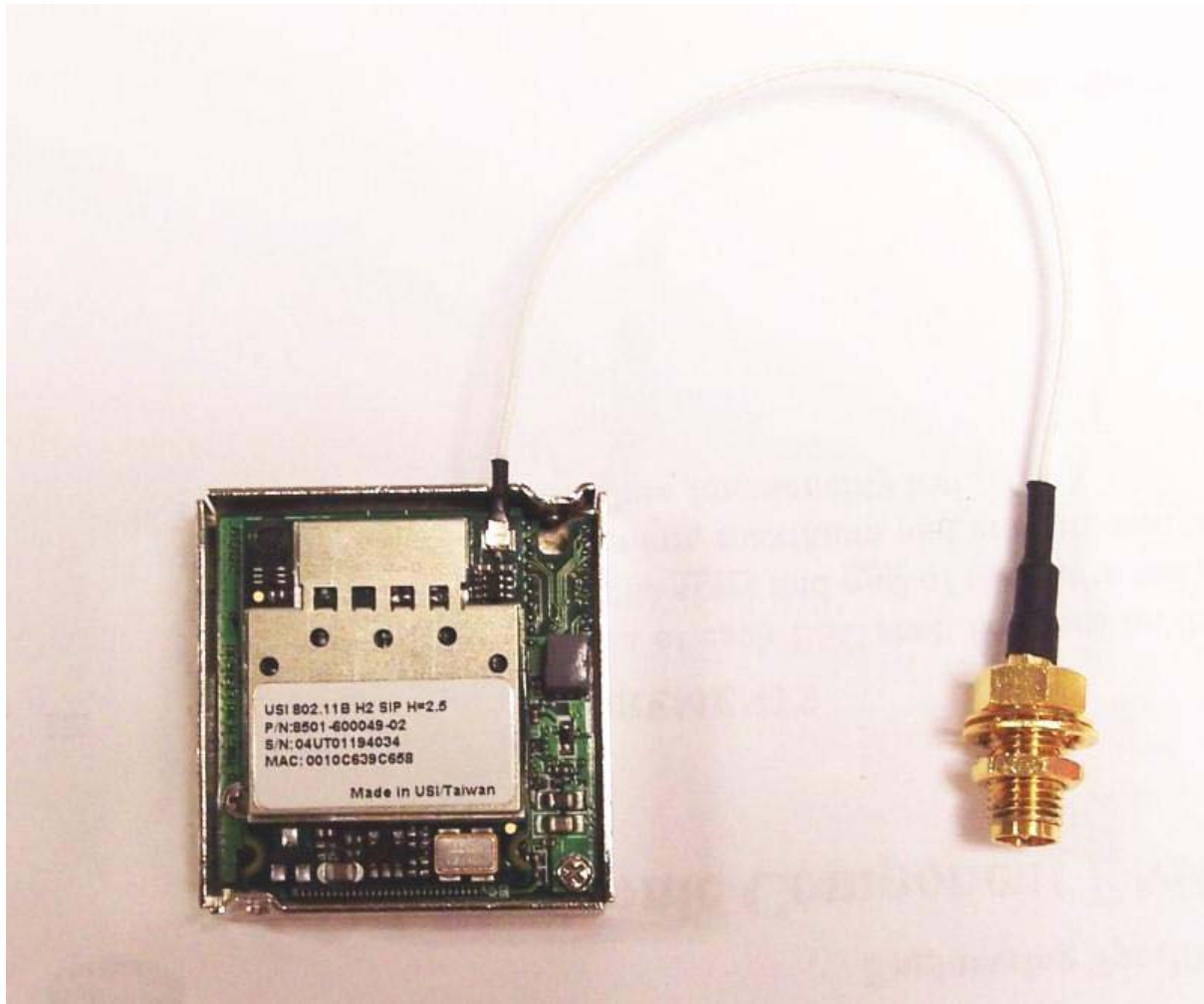
Fig. 6 RF Module – Top shield removed
