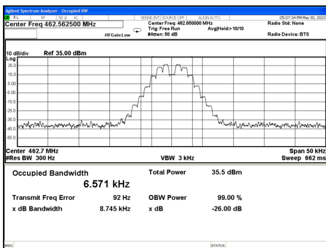
Channel 19: 462.6500MHz
