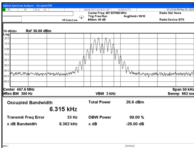
Channel 11: 467.6375MHz
