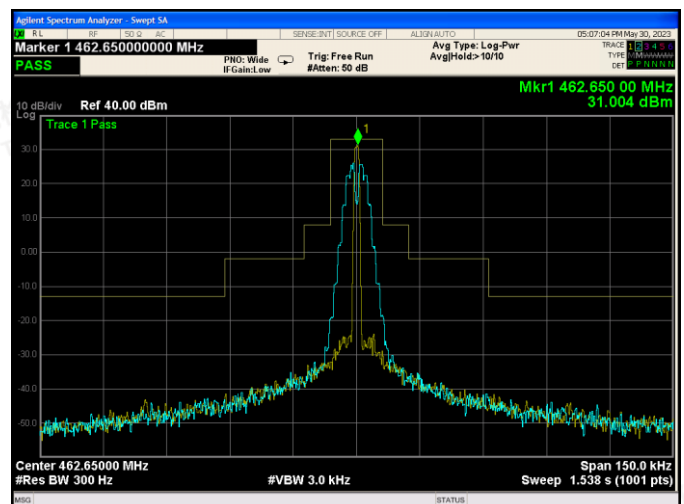
Channel 19: 462.6500MHz
