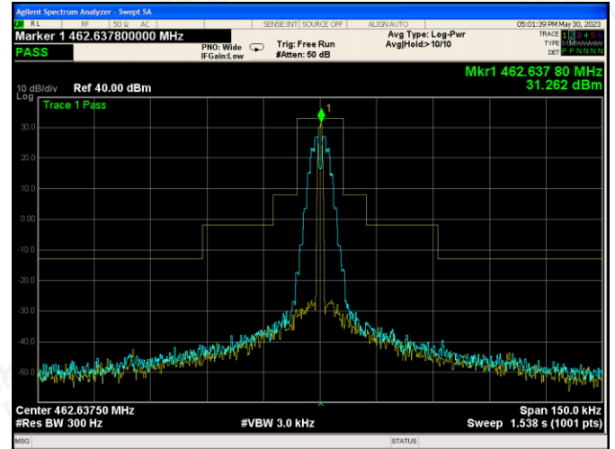
Channel 4: 462.6375MHz
