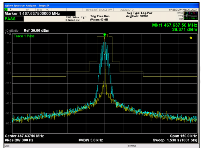
Channel 11: 467.6375MHz
