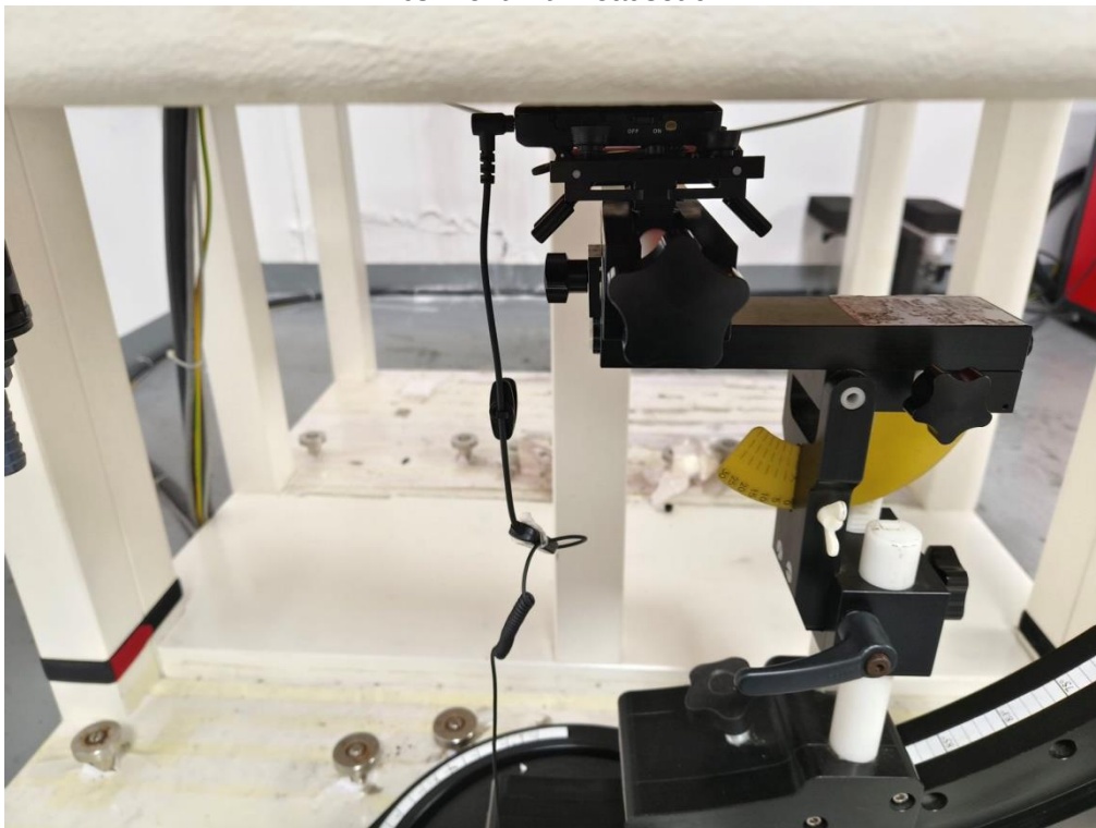
The thickness of EUT is 17mm Limbs Front with headset 0mm
