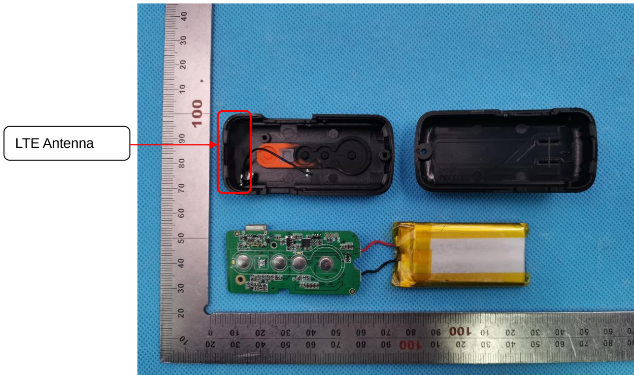
Internal View-1 of EUT
