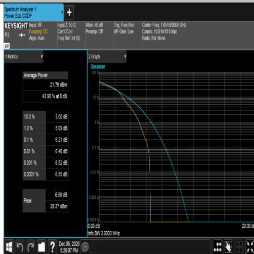
Band2-3MHz-16QAM-18615-1RB#0-PASS
