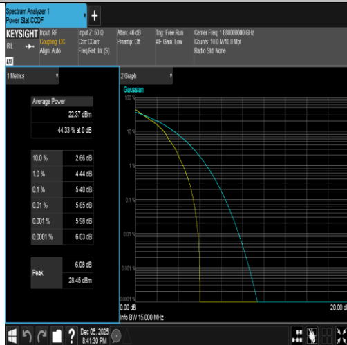
Band2-15MHz-QPSK-18900-1RB#0-PASS
