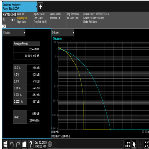
Band2-15MHz-QPSK-18675-1RB#0-PASS
