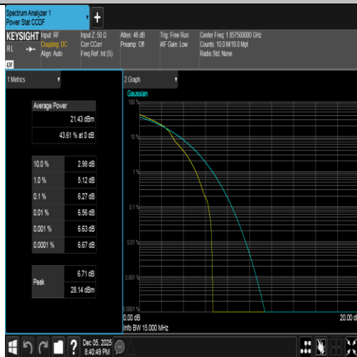
Band2-15MHz-16QAM-18675-1RB#0-PASS
