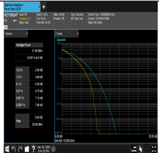
Band2-15MHz-QPSK-18900-75RB#0-PASS
