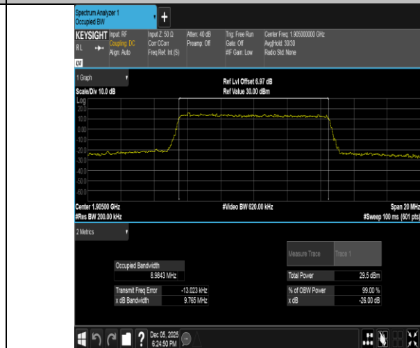
Band2-10MHz-16QAM-19150-50RB#0-PASS
