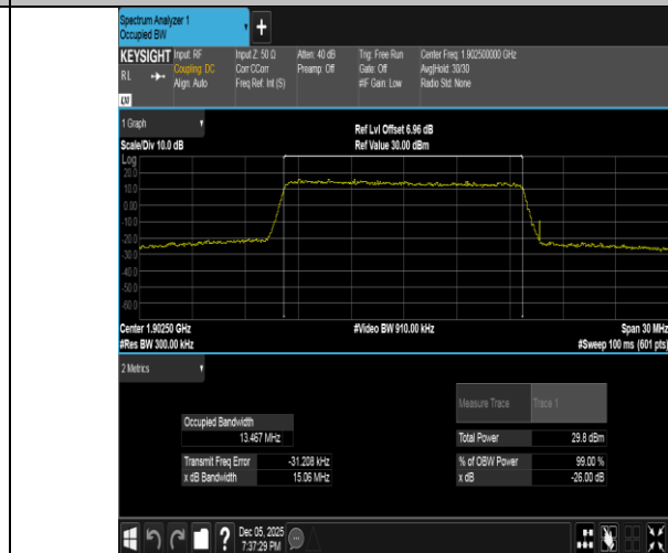
Band2-15MHz-16QAM-19125-75RB#0-PASS
