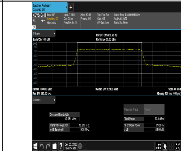
Band2-20MHz-16QAM-18900-100RB#0-PASS
