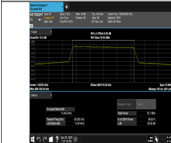
Band2-15MHz-QPSK-19125-75RB#0-PASS
