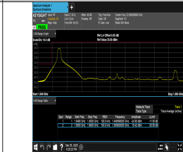
Band2-10MHz-16QAM-18650-1RB#0-PASS
