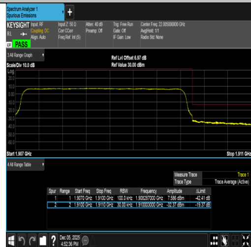
Band2-3MHz-16QAM-19185-15RB#0-PASS
