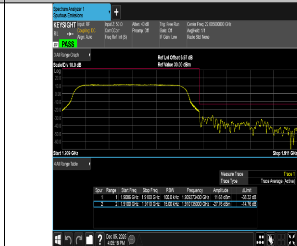
Band2-1.4MHz-16QAM-19193-6RB#0-PASS
