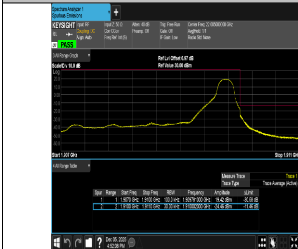
Band2-3MHz-16QAM-19185-1RB#14-PASS
