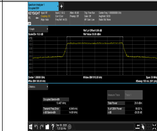
Band2-15MHz-16QAM-18900-75RB#0-PASS
