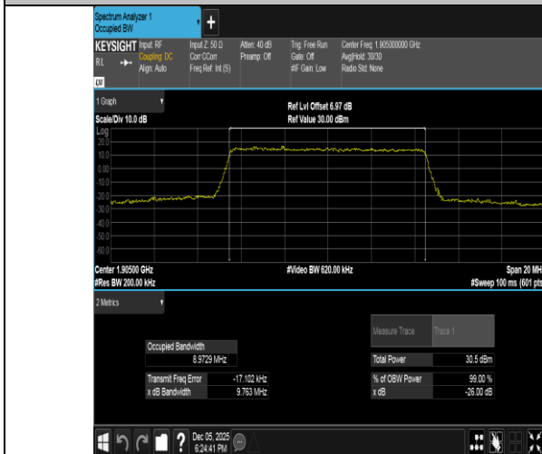
Band2-10MHz-QPSK-19150-50RB#0-PASS
