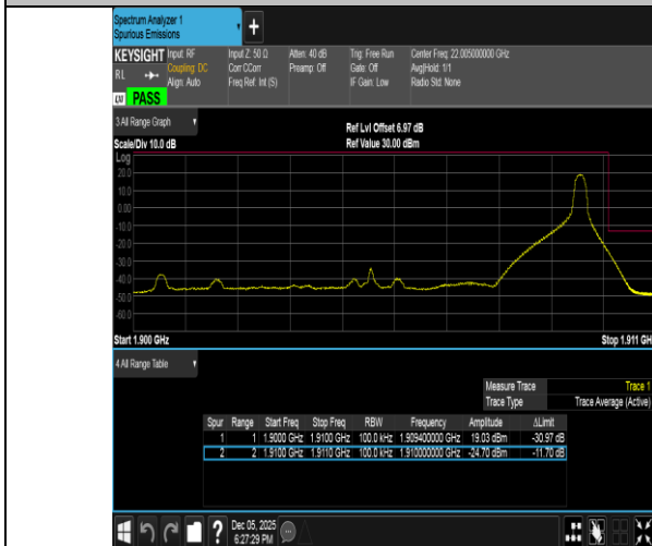
Band2-10MHz-16QAM-19150-1RB#49-PASS
