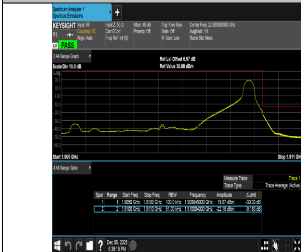
Band2-5MHz-16QAM-19175-1RB#24-PASS
